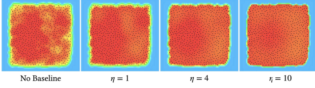
Fig. 5. We visualize the fluid occupancy generated by our transportation optimization with free surfaces for varying sharpness values \eta . The fluid occupancy is shown by a color ramp from blue to red. In the case of no baseline (left), we obtain non-uniform grid volumes inside the fluid with a smeared fluid-air interface. By increasing \eta , the transition near the free surface sharpens and the fluid interior becomes nearly constant.
