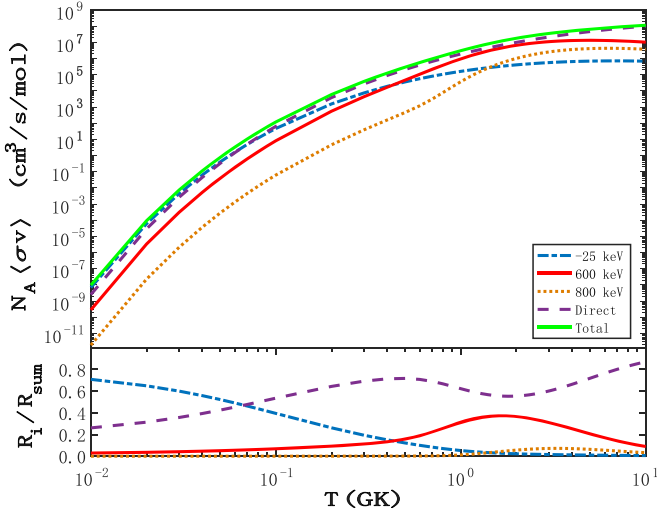
Figure 3. Upper panel: The new reaction rate of {}^7\text{Li}(\text{d},\text{n}){}^4\text{He} as a function of temperature in units of GK is shown by the green solid line. The rate contributions from direct reaction and various resonances are displayed separately. The dashed-dotted line shows the subthreshold resonance ( E_r = -25 keV). The solid red and dotted orange lines correspond to the resonances at E_r = 600 and 800 keV, respectively. The dashed purple line indicates the direct component. Lower panel: This figure shows the contribution ratio from separate components to the total reaction rate.
