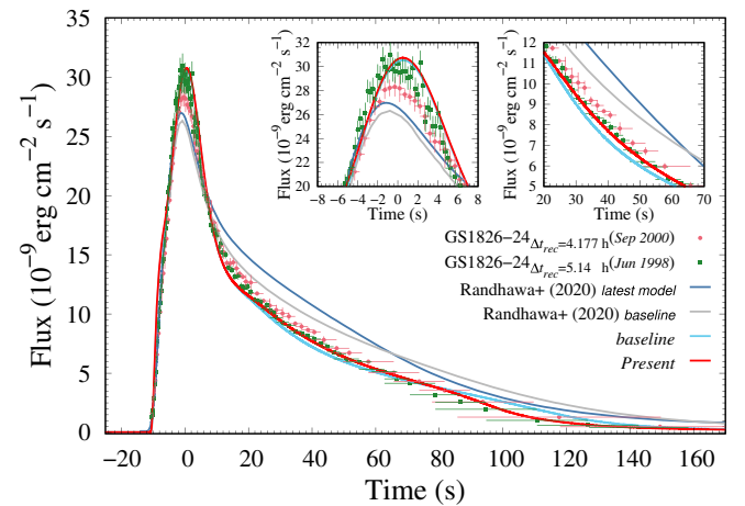
FIG. 3. The best fit baseline and Present modeled light curves to the observed light curve of epoch Jun 1998, and the best fit Randhawa et al. [15] light curves to epoch Sep 2000. The magnified light curves at the burst peak and t = 20 - 70 s are shown in the left and right insets, respectively.
