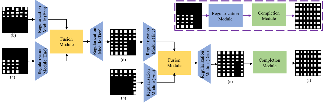
Fig. 2. RFCNet. Two scenarios are shown. For single image facade segmentation (dashed box), it will be processed by Regularization and Completion. For multi-view facade segmentation, Fusion will combine the pairwise latent vector of inputs. (a-c) Multi-view façade segmented images. (d-e) Intermediate fused façade images. (f) Final synthetic output of RFCNet.
