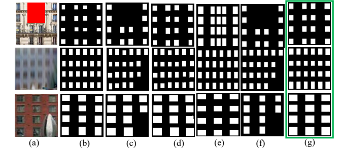
Fig. 8: Regularization and Completion Qualitative Comparison. (a) Occluded facade images from ECP, WVS and GSV respectively. (b) Ground Truth. (c) Initial Segmentation. (d) Segmentation completed by DeepFill. (e) IPM results. (f) Our Regularization. (g) Our Regularization and Completion. Note: We manually mask ECP facade images shown in red box.
