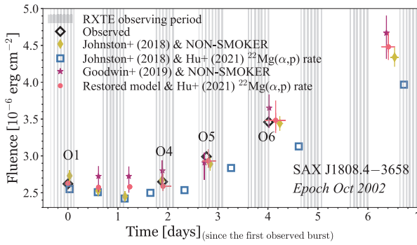
Figure 2. The bursts' fluences and times of the SAX J1808.4–3658 PRE burst, recorded by the Rossi X-ray Timing Explorer (RXTE) [1], based on Johnston et al. [6] and Goodwin et al. [7] models with NON-SMOKER ^{22}\text{Mg}(\alpha, p) reaction rate, and the restored Johnston et al. model with Hu et al. ^{22}\text{Mg}(\alpha, p) reaction rate [8]. The light curves of observed (and modeled) bursts O1 (B1), O4 (B4), O5 (B5), and O6 (B6) are plotted in Fig. 1.
