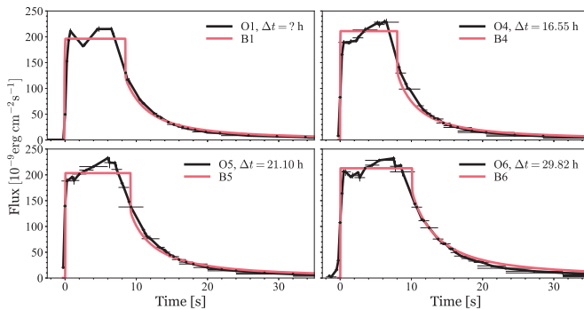
Figure 1. SAX J1808.4–3658 PRE bursts of Epoch Oct 2002. The observed bursts O1, O4, O5, and O6 (black lines), and the corresponding modeled bursts B1, B4, B5, and B6 (red lines) based on the restored Johnston et al. [6] model using Hu et al. ^{22}\text{Mg}(\alpha, p) reaction rate [8] with mass fractions X_{\text{H}}/X_{\text{He}} = 0.413/0.567 and time dependent accretion rate.
