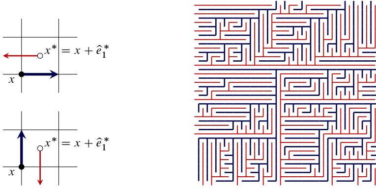
Fig. 4.1. Left plot: An illustration of the duality relation between the edges of \mathcal{G}_{\xi\Box} (black/thick) and those of \mathcal{G}_{\xi\Box}^* (red/thin). Right plot: An illustration of a (blue/thick) north-east directed geodesic graph \mathcal{G}_{\xi\Box} and its (red/thin) south-west directed dual \mathcal{G}_{\xi\Box}^* .
