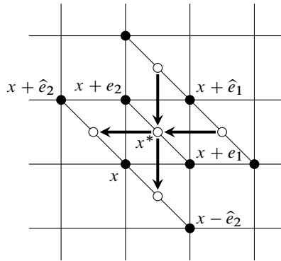
Fig. 4.5. The flow of Busemann measure follows the arrows. The antidiagonal edge (x + e_1, x + e_2) is identified with the dual point x^* = x + \hat{e}_1^* . The Busemann measure \mu_{x+e_1, x+e_2} on this edge is composed of the mass flowing from the north and east, and it in turns divides its mass between the flows south and west.
