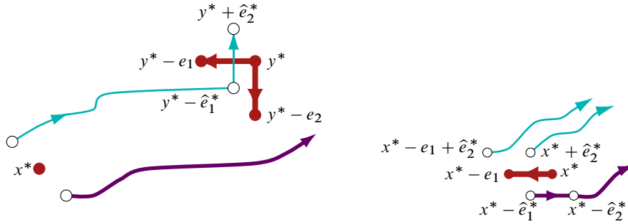
Fig. 8.1. The proofs of Lemma 8.2 (left) and Theorem 4.3 (right). \zeta -geodesics are in green and thin. \eta -geodesics are in purple with medium thickness. Directed edges in \mathcal{G}_{\cup[\zeta, \eta]}^* are in red/thick. White circles are points in \mathbb{Z}^2 while points in \mathbb{Z}^{2*} are filled in (red).
