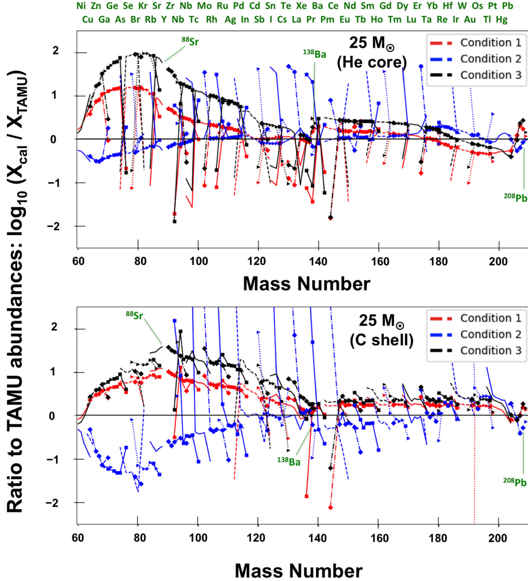
FIG. 15. Ratios of calculated s -process abundances to TAMU abundances for the 25 M_{\odot} (see Fig. 12) using ^{22}\text{Ne}(\alpha, n) and ^{22}\text{Ne}(\alpha, \gamma) rates in which strength of some resonances are changed. See text for details. Isotopes of the same elements are connected by adjoining lines [some key s -process peak isotopes ( ^{88}\text{Sr} , ^{138}\text{Ba} , and ^{208}\text{Pb} ) are labeled for clarification].
