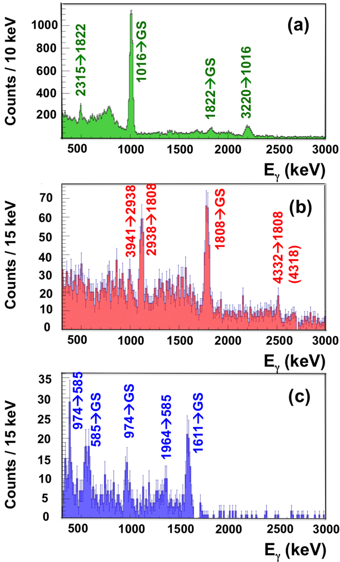
FIG. 8. (a) \gamma -ray spectrum from {}^{22}\text{Ne}(d, p\gamma){}^{23}\text{Ne} reaction in coincidence with E_x = \text{GS to } 5 \text{ MeV} from the proton excitation-energy spectrum. (b) \gamma -ray spectrum from the {}^{22}\text{Ne}({}^6\text{Li}, d\gamma){}^{26}\text{Mg} reaction in coincidence with E_x = 4\text{--}11.5 \text{ MeV} . (c) \gamma -ray spectrum from the {}^{22}\text{Ne}({}^6\text{Li}, dn\gamma){}^{25}\text{Mg} reaction in coincidence with E_x({}^{26}\text{Mg}) = 11.0\text{--}14.0 \text{ MeV} deuterons.
