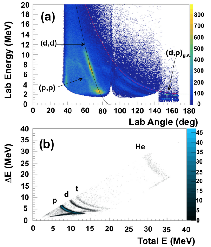
FIG. 2. (a) Energy versus scattering angle plot from ^{22}\text{Ne} + \text{CD}_2 . Theoretical elastic ( d, d ) and ( d, p ) ground state kinematic lines are shown together. The elastic ( p, p ) line is because of contaminants in the target. (b) E - \Delta E plot from a Barrel detector, where protons, deuterons, tritons, and He are observed.
