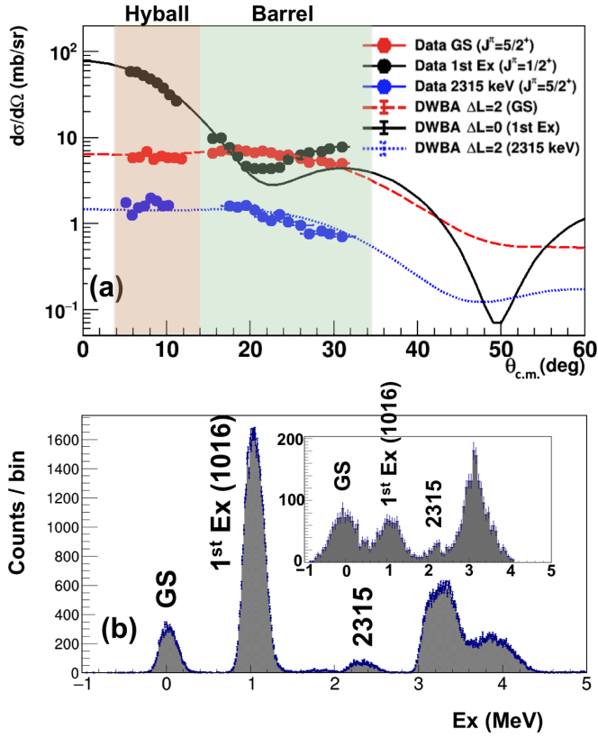
FIG. 3. (a) Angular differential cross sections of ^{22}\text{Ne}(d, p) reactions for populating low-lying states of ^{23}\text{Ne} . (b) Excitation spectra of ^{23}\text{Ne} from the Hyball at \theta_{\text{c.m.}} = 5\text{--}12^\circ (whole detector). Inset: Barrel at \theta_{\text{c.m.}} = 18\text{--}19^\circ .
