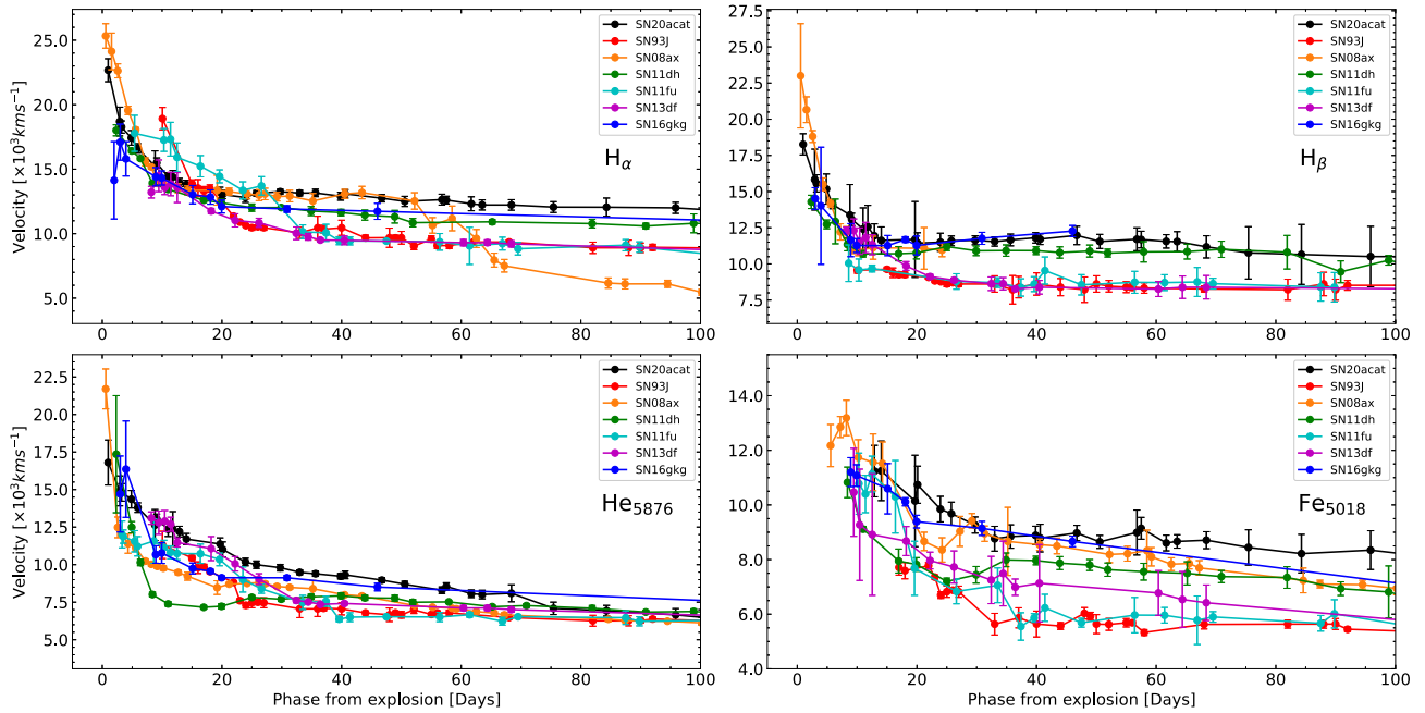
Figure 9. Line velocity evolution of the H\alpha , H\beta , He\ I\ \lambda 5876 , and Fe\ II\ \lambda 5018 lines for SN 2020acat, which are compared to those of other SNe I Ib, over the first 100 d from explosion. It's clearly seen that SN 2020acat displays one of the highest line velocities of the SNe shown here.
