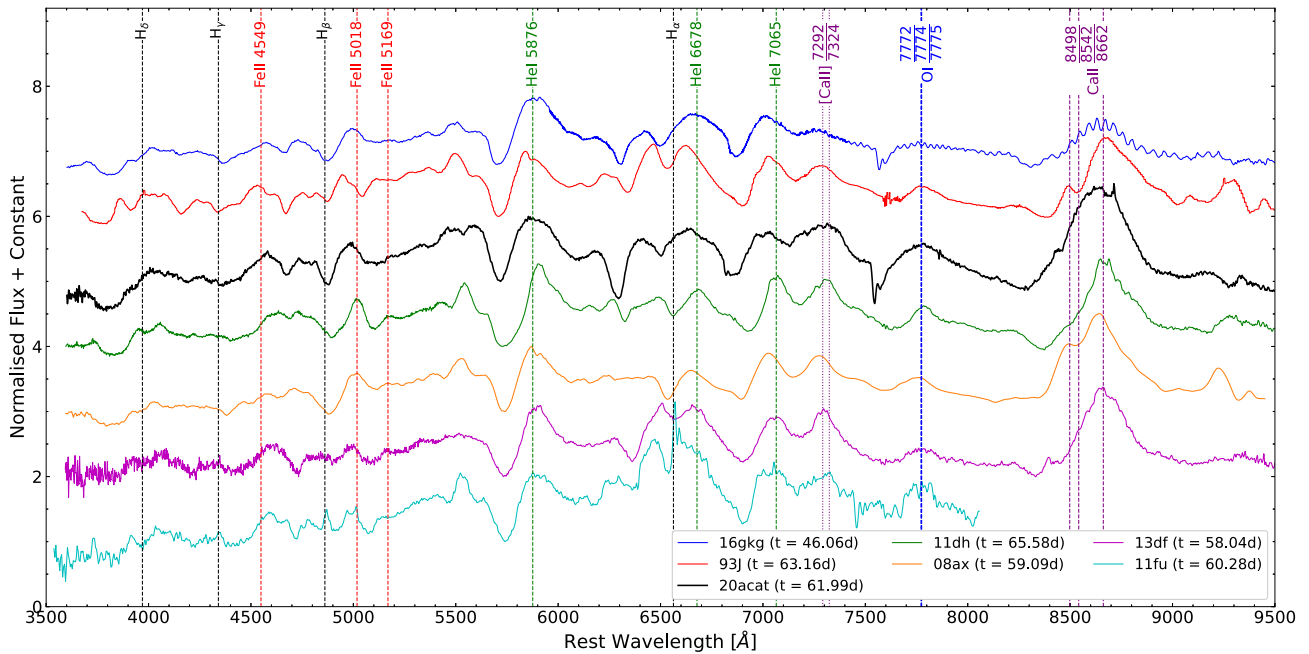
Figure 10. Spectral comparison of SN 2020acat with several well-observed SNe I Ib roughly 60 d after their reported explosion date. All spectra are shown in the rest frame and are ranked in terms of He I \lambda 5876 line velocity. Key transition phase element lines are marked at their rest wavelength, with allowed transitions shown as the dashed lines and forbidden lines shown as dotted lines.
