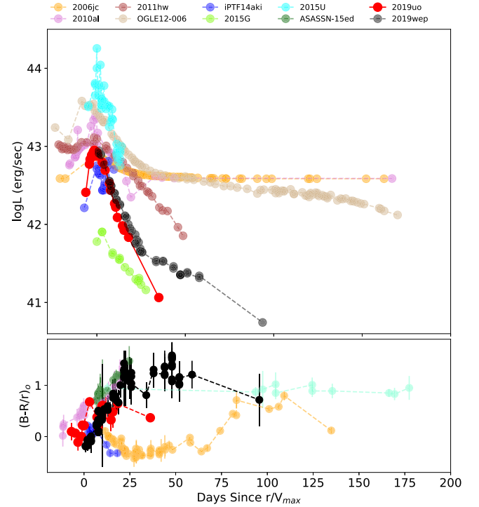
Figure 4. Complete bolometric light curve and B-R/r color curve of SN 2019wep. The comparison sample includes SNe 2006jc (Pastorello et al. 2007; Foley et al. 2007), 2010al (Pastorello et al. 2015b), OGLE-SN-006 (Pastorello et al. 2015e), 2011hw (Pastorello et al. 2015b), iPTF14aki (Hosseinzadeh et al. 2017), 2015U (Shivvers et al. 2016; Hosseinzadeh et al. 2017), 2015G (Hosseinzadeh et al. 2017), ASASSN-15ed (Pastorello et al. 2015c), and 2019uo (Gangopadhyay et al. 2020a).
