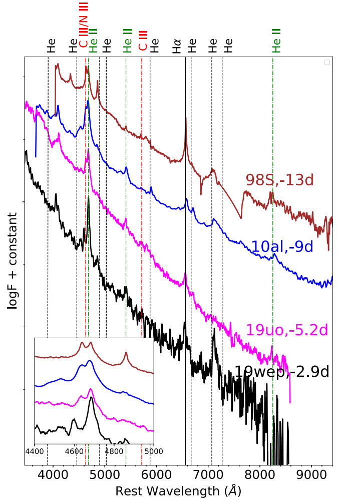
Figure 7. Spectral comparison of SN 2019wep at -2.9 days with SNe 1998S (Fassia et al. 2001), 2010al (Pastorello et al. 2015b), and 2019uo (Gangopadhyay et al. 2020a). Prominent flash ionization features are marked.
