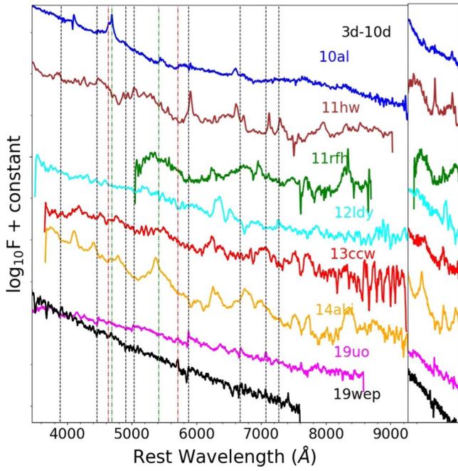
Figure 8. Comparison of the spectrum of SN 2019wep to other SNe Ibn. SN 2019wep belongs to the P cygni subclass and shows a close resemblance to SNe 2010al and 2019uo. The data for this are taken from SNe 2010al (Pastorello et al. 2015a), 2011hw (Pastorello et al. 2015a), PTF11rfh (Hosseinizadeh et al. 2017), PTF12ldy (Hosseinizadeh et al. 2017), LSQ13ccw (Pastorello et al. 2015b), iPTF14aki (Hosseinizadeh et al. 2017), and 2019uo (Gangopadhyay et al. 2020a). The right panel of the plot shows the P cygni and the emission lines of the He I 5876 Å feature.
