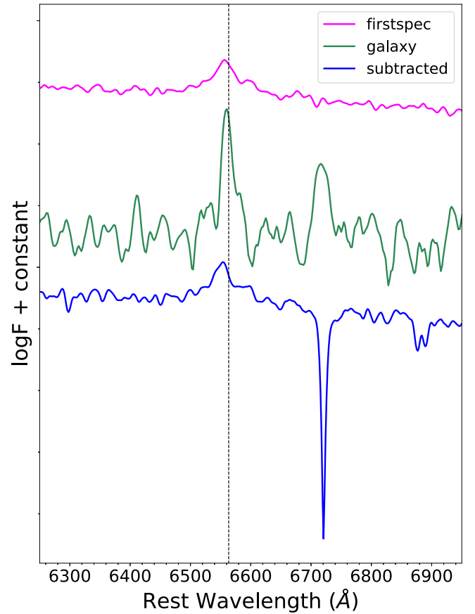
Figure 13. The first day, galaxy and subtracted spectra of SN 2019wep taken with the LCO networks. A reminiscent H\alpha is seen in the subtracted profile.
