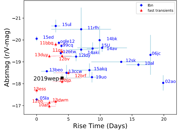
Figure 3. The \Delta m_{15} vs. rise time (left panel) and absolute magnitude vs. rise time (right panel) correlation plots of SN 2019wep with a sample of SNe Ibn and fast transients. The sample of type SNe Ibn has been taken from Hosseinzadeh et al. (2017) and Gangopadhyay et al. (2020a) and the sample of fast transients are taken from Drout et al. (2014).
