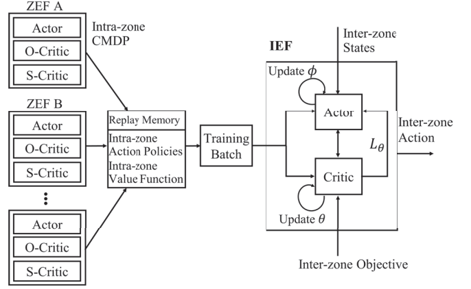
Fig. 7. Collective Actor-Critic DRL.
