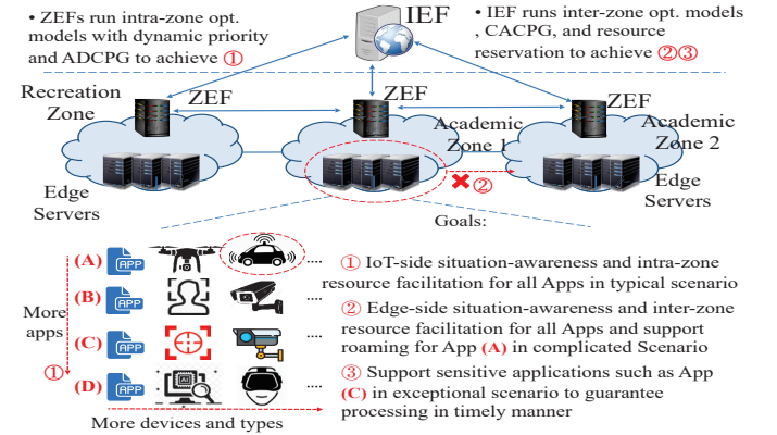
Fig. 3. Intelligent, hierarchical, and adaptive facilitation mechanism.
