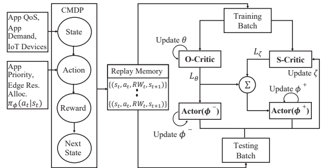
Fig. 5. The ADCPG DRL scheme.
