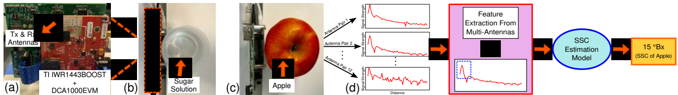
Figure 1: (a) SSCense uses a millimeter-wave (mmWave) transceiver with 3 transmitters and 4 receivers to estimate the Soluble Sugar Content (SSC) of fruits; (b) Top-down view of data collection setup for controlled experiments with sugar solutions inside a container; (c–d) Fruits are positioned in front of the transceiver, and reflected signals from multiple antenna pairs are collected. The extracted features from these signals are fed to an estimation model for predicting SSC on a °Brix scale [1].
