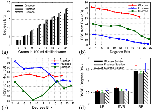
Figure 2: (a) Measured °Bx of glucose, fructose, and sucrose solutions; (b) The RSS from Rx4 decreases as SSC increases; (c) But no relation found between RSS from Rx3 and SSC; (d) Regression models developed using data samples from three sugar solutions.
