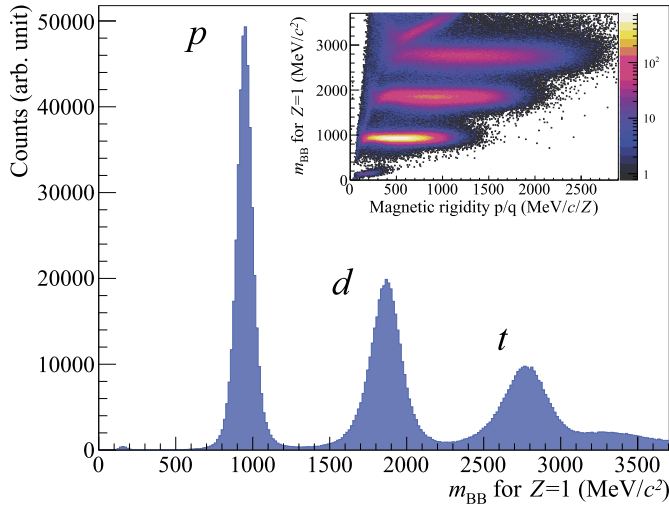
Fig. 1. Mass spectrum around Z = 1 particles in central collisions of the ^{132}\text{Sn}+^{124}\text{Sn} system obtained with the S \pi RIT-TPC and a two-dimensional plot of mass vs. magnetic rigidity magnitude in the right-top panel. The mass m_{\text{BB}} was obtained as the solution of the equation in the text.
