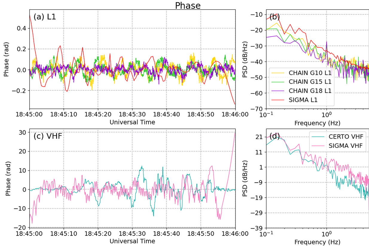
Fig. 5. Signal phase time series and PSDs of both observed and simulated data for L1 (panels a and b) and VHF (panels c and d). Note that the L1 signal is absolute phase while the VHF signal is relative phase.
