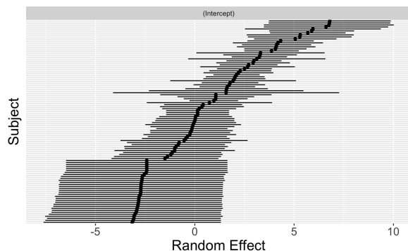
Figure 6: By-participant intercepts.
