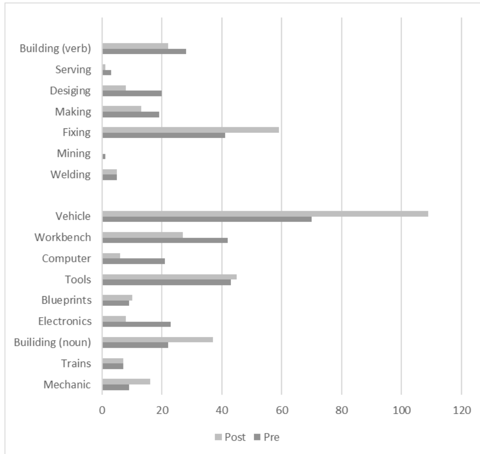
Figure 2: Nouns and verbs associated with the DAET
