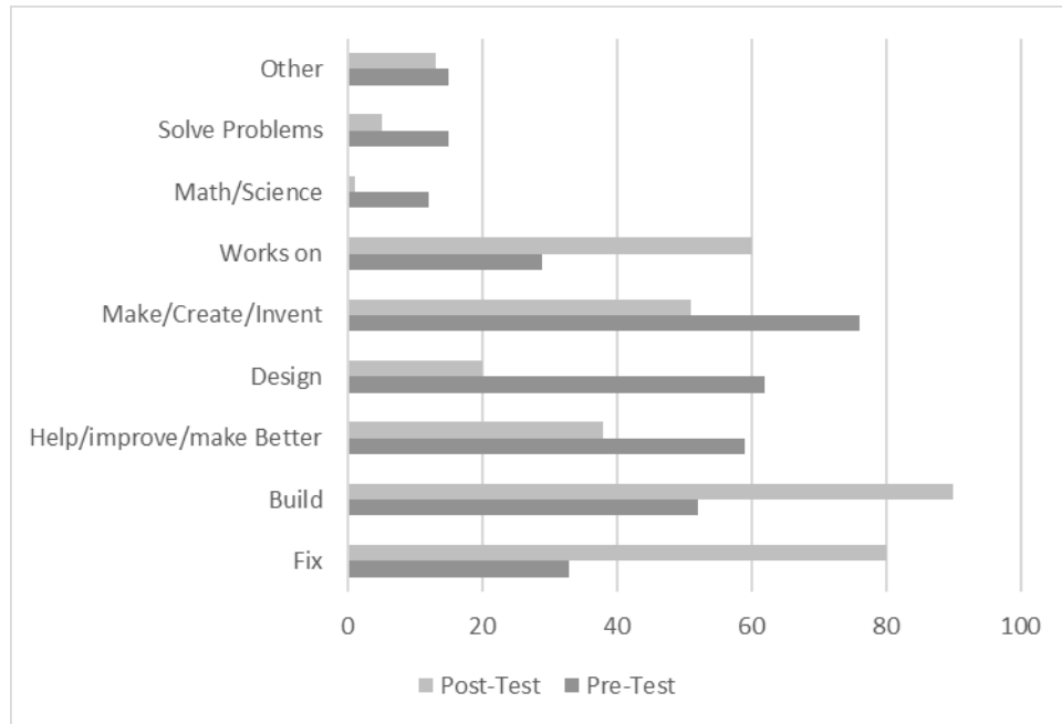
Figure 1: Responses to open-ended question on what engineers do
