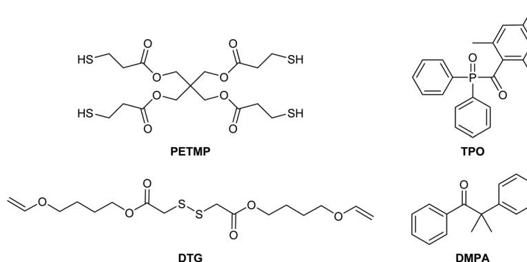
Fig. 4 Monomers (PETMP and DTG) and photoinitiators (TPO and DMPA) used to study stress relaxation in thiol–ene disulfide networks. TPO is initiated by visible light at 405 nm and DMPA is initiated by UV light at 365 nm.
