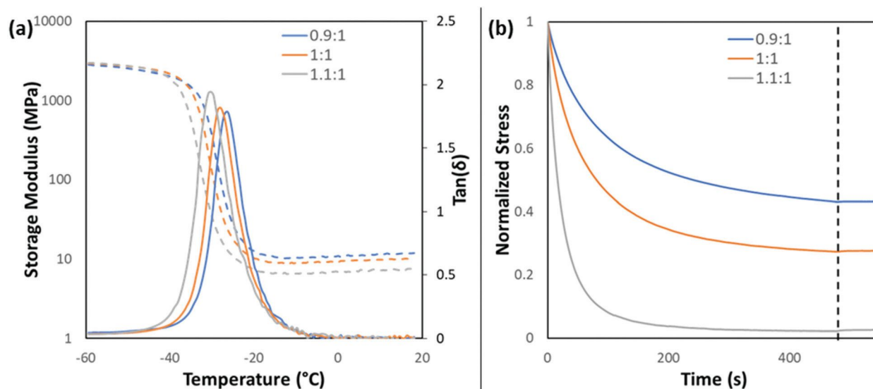
Fig. 5 (a) Dynamic mechanical analysis of the 0.9 : 1, 1 : 1, and 1.1 : 1 stoichiometry networks. The \tan(\delta) is shown as a solid line and the storage modulus is shown as a dashed line for each formation, and (b) the normalized stress over time, for 0.9 : 1, 1 : 1, and 1.1 : 1 ratios of thiol to alkene with 3.5 wt% DMPA as a UV photoinitiator at 15 \text{ mW cm}^{-2} . The vertical dashed line indicates the time at which the light was turned off during the experiment.
