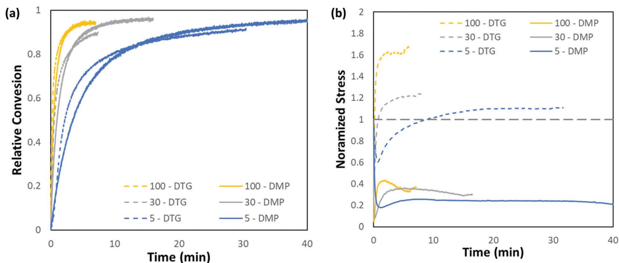
Fig. 11 For samples of PETMP with either DTG (dashed) or DMP (solid) with a 0.5 : 1 ratio of thiol to alkene, (a) relative conversion of alkene over time during the disulfide–ene polymerization at various light intensities ( \text{mW cm}^{-2} ), where zero conversion corresponds to the initial conversion reached after the first stage thiol–ene reaction, and (b) the normalized stress during the disulfide–ene polymerization for samples cured through the disulfide–ene reaction at various light intensities ( \text{mW cm}^{-2} ). Samples were first cured using 14 \text{ mW cm}^{-2} 405 nm light until the film was cured enough to cut and handle.
