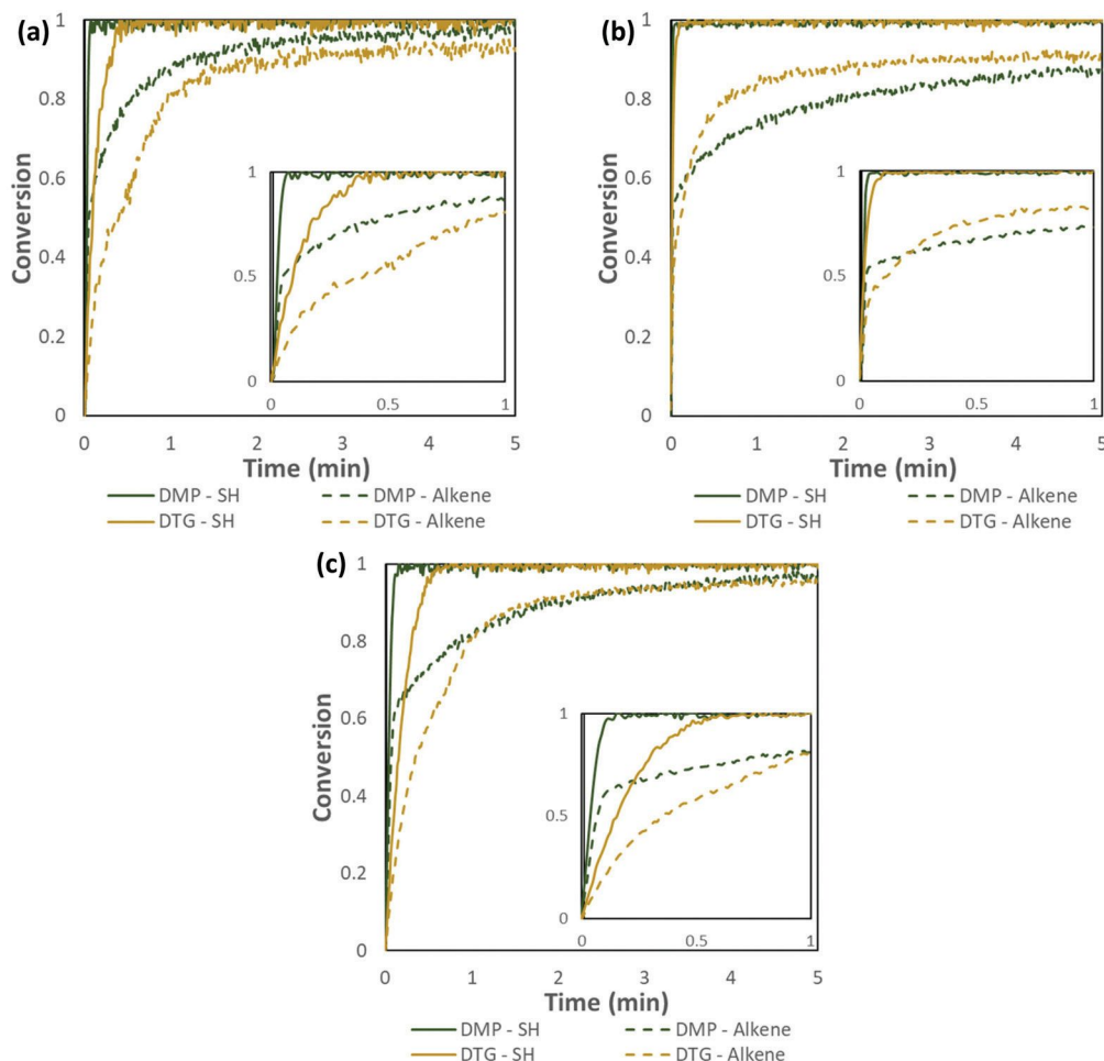
Fig. 8 Thiol and vinyl conversion over time for the two disulfide-containing divinyl ether monomers copolymerized with thiols of different thiyl radical stability: (a) PETMP, (b) PETTG, and (c) SiTSH. The insets show the first minute of the polymerization for each thiol to emphasize the difference in the thiol–ene rate for each thiol–disulfide pair.
