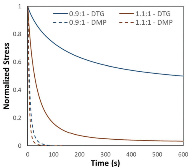
Fig. 10 The normalized stress over time for DTG (solid) and DMP (dashed) at two ratios of thiol to alkene. Samples were prepared with 3.5 wt% DMPA, stretch to 8% strain, and exposed to 15 \text{ mW cm}^{-2} 365 nm light.
