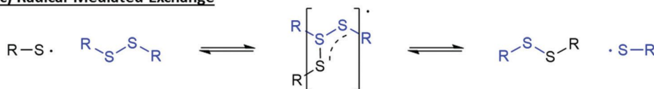
Fig. 1 Schematic of several dynamic mechanisms of disulfide bonds: (a) metatheses, (b) reversible addition via homolytic cleavage and recombination of disulfide bonds, and (c) radical-mediated reversible exchange between thiyl radicals and disulfides.
