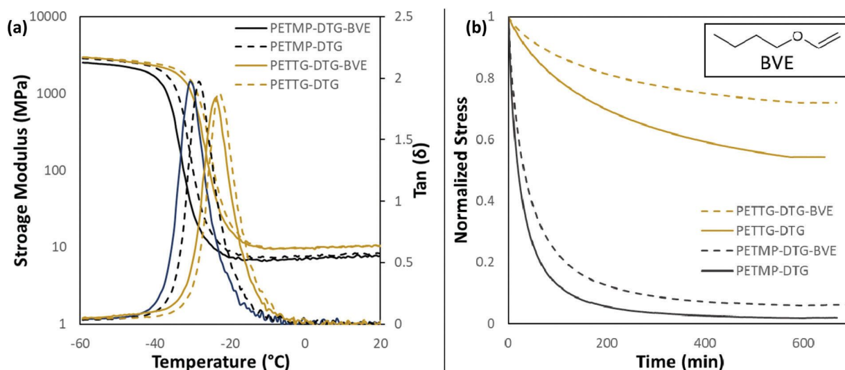
Fig. 9 (a) DMA trace and (b) stress relaxation of each network, with butyl vinyl ether included in the top right. Each network was made with a 1.1:1 ratio of thiol to alkene and was cured into a 250 μm films with 1 wt% TPO irradiated with 405 nm light at 20 mW cm -2 for 5 minutes on each side. Stress relaxation was done with 3.5 wt% DMPA and 365 nm light at 15 mW cm -2 for 10 minutes at 8% strain.
