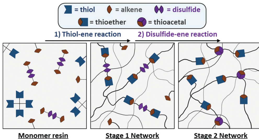
Fig. 3 Schematic of the thiol-ene-disulfide polymerization for a multifunctional thiol with a disulfide containing divinyl ether (alkene). Polymerization proceeds, beginning with a monomer resin mixture to form a primarily thiol-ene stage 1 network made up of thioether bonds, then through the disulfide-ene reaction to form the thioacetal bonds in the stage 2 network.
