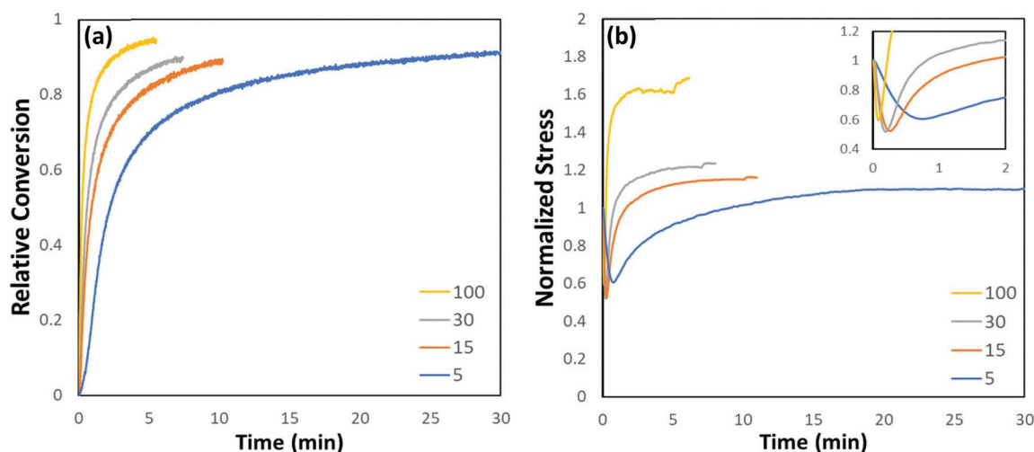
Fig. 6 For PETMP-DTG with a 0.5 : 1 ratio of thiol to alkene, (a) relative conversion of alkene over time at various light intensities ( \text{mW cm}^{-2} ), where zero conversion corresponds to the initial conversion reached after the first stage thiol–ene reaction, and (b) the normalized stress during the disulfide–ene polymerization for samples cured through the disulfide–ene reaction at various light intensities ( \text{mW cm}^{-2} ). The inset highlights the initial drop in stress for each light intensity. Samples were first cured using 14 \text{mW cm}^{-2} 405 nm light until the film was just cured enough to cut and handle.
