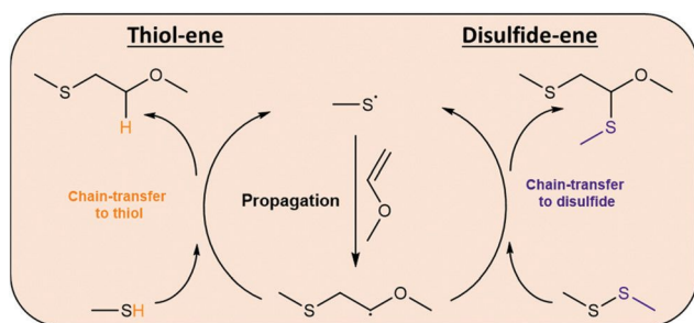
Fig. 2 Mechanism of thiol-ene disulfidation polymerization, where both reactions share a propagation step but have distinct chain transfer pathways.
