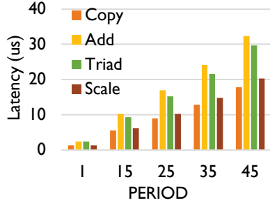
Figure 2: Latency measured by STREAM for varying delay injection.
