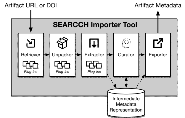
Figure 3: The SEARCCH importer tool uses modules to obtain metadata about artifacts stored in a variety of locations and formats.
