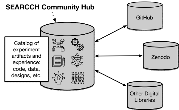
Figure 1: SEARCCH catalogs metadata about cybersecurity artifacts that are stored in separate repositories.
