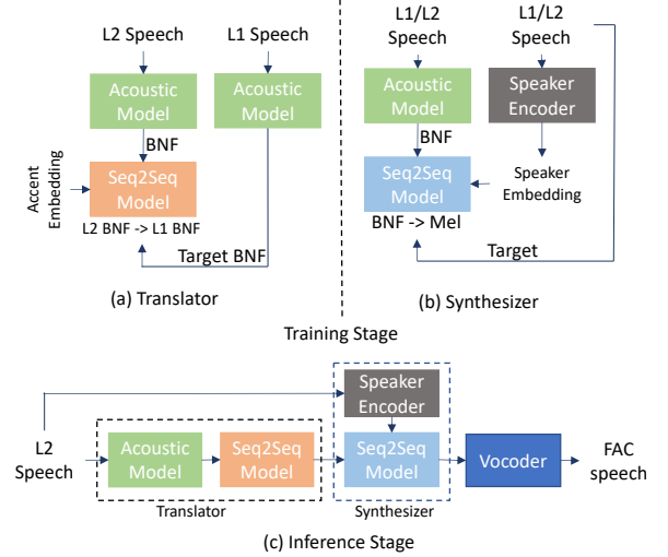
Figure 1: Training workflow for (a) the translator and (b) the synthesizer. (c) Overall inference workflow of the system.
