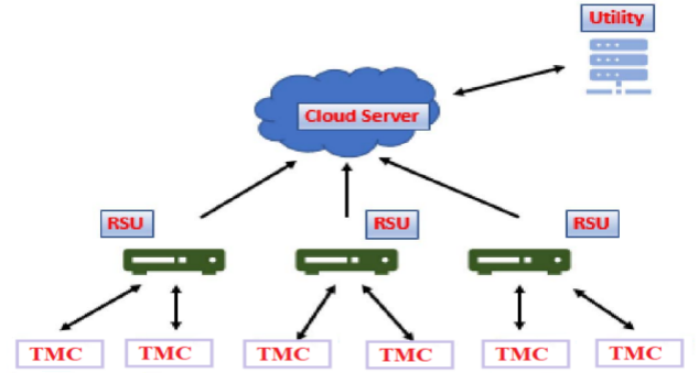
Figure 1: Architecture of a Smart Transportation System.
