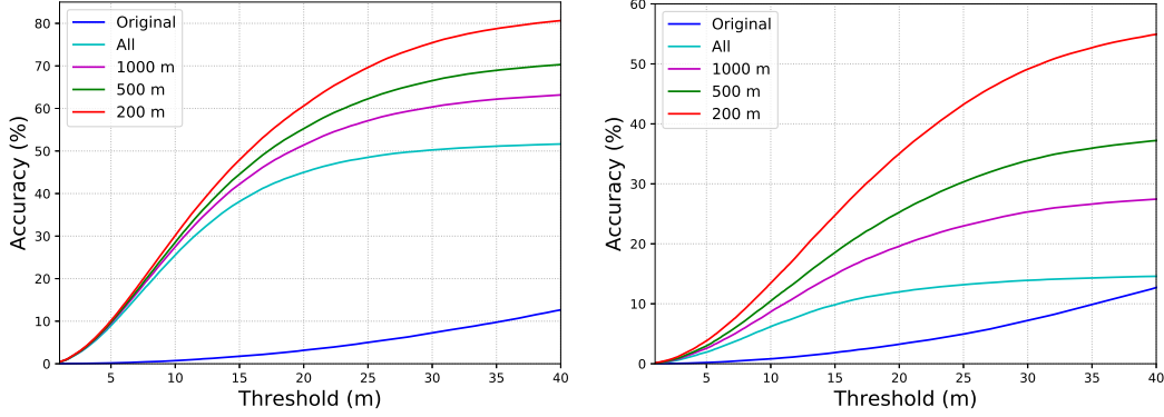
Figure 9. Same-area (left) and cross-area (right) meter-level localization accuracy of different search scopes given noisy GPS signal.
