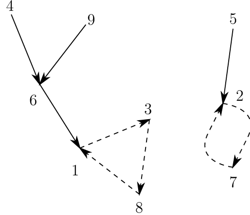
Figure 1: Example of the mapping directed graph of f . In this example, f(1) = 3, f(2) = 7, f(3) = 8, f(4) = 6, f(5) = 2, f(6) = 1, f(7) = 2, f(8) = 1 and f(9) = 6 . Also \mathcal{M} = \{1, 2, 3, 7, 8\} .
