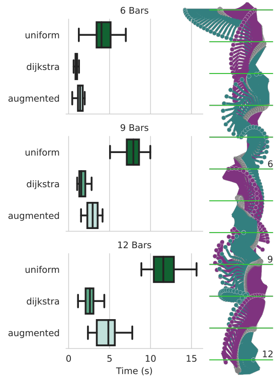
Fig. 11. Timing results for three “long monkey” domains. On the right the “12 Bars” version of the environment is shown, along with the swept volume of by an example multi-modal plan. On the left, timing results for “6 Bars,” “9 Bars,” and “12 Bars” are shown for Uniform , Dijkstra , and Augmented —each box plot represents 30 trials. Note that as the problems become more challenging (i.e., there are more bars and thus a longer sequence of transitions needed), the benefits of using the discrete leads become more pronounced. In this scenario the specificity of Augmented does not provide any benefits over Dijkstra , as the location of the grasps matters less than the sequence.
