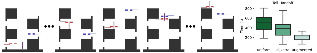
Fig. 14. Timing results for the “tall handoff” domain. On the left, five stills are shown from a multi-modal plan in this domain. The start and goal are shown on the far left and right respectively. The end-effectors are red and blue, the graspable object is purple. An example of a necessary regrasp to achieve a handoff is shown in the middle. Timing results are shown on the right, 30 trials for each planner. Even in difficult TAMP-like scenarios, Augmented learns important information about feasibility to make search more efficient. Uniform had four failures given 1200 seconds, which are not included in the box plot.
