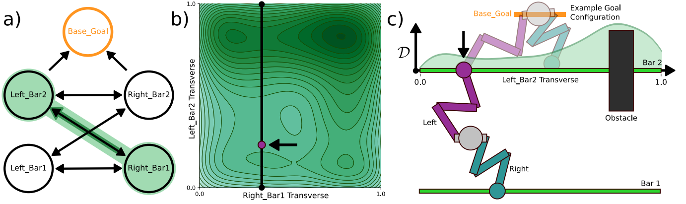
Fig. 7. Visualization of transition graph weights. a) A transition graph for the “simple monkey” domain. The transition from grasping bar 1 with the right limb (“Right_Bar1”) to grasping bar 2 with the left limb (“Left_Bar2”) is highlighted. b) A contour map of the weights for the highlighted transition (gathered offline). The co-parameter for grasping bar 1 with the right limb is plotted on the X-axis, while the co-parameter of grasping bar 2 with the left limb is plotted on the Y-axis. Darker shading represent higher-weight (transitions we expect to be difficult). A slice for a specific X-axis co-parameter (i.e., initial placement of the right gripper) is marked in black, and shown in c) . c) The “simple monkey” domain, with the weights of the slice from b) visualized over bar 2. The left arm of the robot is shown grasping bar 2 (highlighted by the arrow), and thus is a transition configuration. The transition is marked at its co-parameters by a purple point in b) . To reach “Base_Goal,” the robot must grasp bar 2, visualized as an orange region for the base and an example satisfying configuration.
