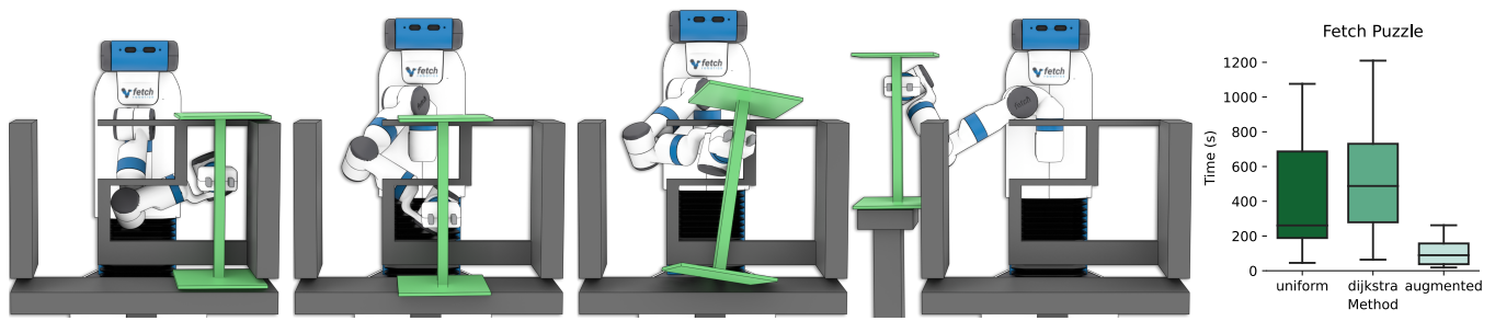
Fig. 17. A complicated “puzzle” domain for the Fetch block stacking problem. Here, a dumbbell-shaped object can be grasped anywhere along its spine. The Fetch must move the dumbbell from the initial configuration to the middle of the box, so it can be regrasped from the top to be extracted from the box. Similar to Fig. 14, given the importance of grasp and placement location, Augmented outperforms the other methods. Timing results represent 30 trials.
