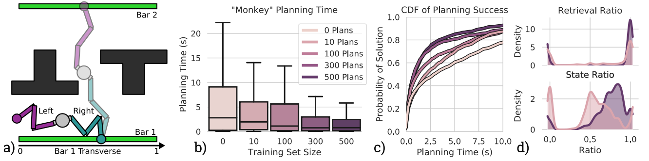
Fig. 8. a) A two-limbed “monkey” robot must grasp the other bar. Start configurations are sampled such that the robot grasps the first bar. The location of the robot’s grasp on the bar corresponds to the co-parameter of the foliation, indicated below the bar. b) Timing results for 500 trials are presented. On the x -axis, we show results for ALEF trained on increasing numbers of training paths. We achieve significant speed-up given only a few examples. c) Cumulative probability of finding a solution versus time. Our method solves more problems faster as experience is gathered. d) Retrieval ratio and valid state ratio for ALEF trained on 10 and 500 examples. More paths are retrieved and the number of relevant experiences increases given more training data.
