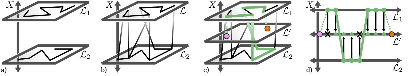
Fig. 4. Sketch of ALEF, the proposed method. a) Valid paths from different action parameterizations are gathered as experience. These paths exist in the leaves \mathcal{L}_1 and \mathcal{L}_2 of the foliated manifold of the action. Note that these are paths in the configuration space, but are such that each configuration satisfies their leaf’s constraint. b) ALEF builds a sparse roadmap in the augmented foliated space (AFS, Sec. IV-A), finding feasible connections across leaves. Connections are such that the foliation constraint is always satisfied. c) Upon retrieval for a query in new leaf \mathcal{L}' , a path is found in the roadmap (highlighted) given a start and goal (pink and orange circles). d) This path is projected to \mathcal{L}' . Valid configurations are used as samples in the new query.
