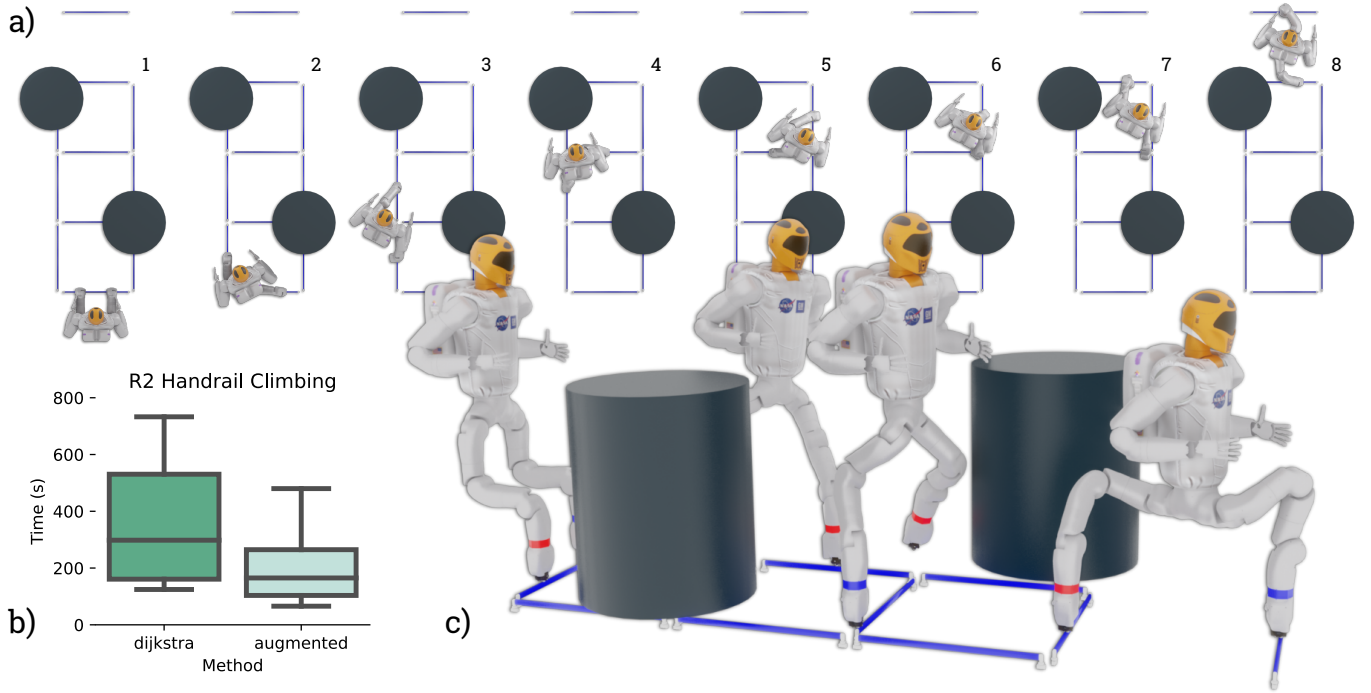
Fig. 13. Timing results for NASA’s Robonaut 2 climbing in a handrail domain with obstacles. a) shows the sequence of transition states found in one trial of the multi-modal planner. b) shows timing results for 30 trials of both Dijkstra and Augmented . Uniform was unable to solve this problem with 1200 seconds per trial for all 30 trials. Augmented achieves more consistent performance due to learning to avoid obstacles and challenging transitions. c) shows another view of the same trial shown in a) .
