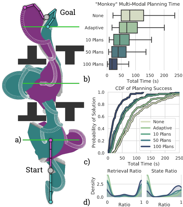
Fig. 9. a) The swept volume of a multi-modal plan. The start configuration and an example goal configuration are highlighted. b) Total multi-modal planning time for 100 trials for each method, including training time for ALEF. Obstacles vary in position and rotation between each query. Shown are a baseline method with no experience (“None”), ALEF which learns from an empty roadmap (“Adaptive”), and ALEF trained on n multi-modal queries (“ n plans”). Starting with an empty roadmap, our method provides a small benefit over the baseline. Training from prior queries gives substantial benefit for multi-modal planning. c) Timing results presented as a cumulative distribution curve. d) Retrieval and valid state ratios for all motion planning queries. ALEF retrieves more relevant experience as its training set increases.
