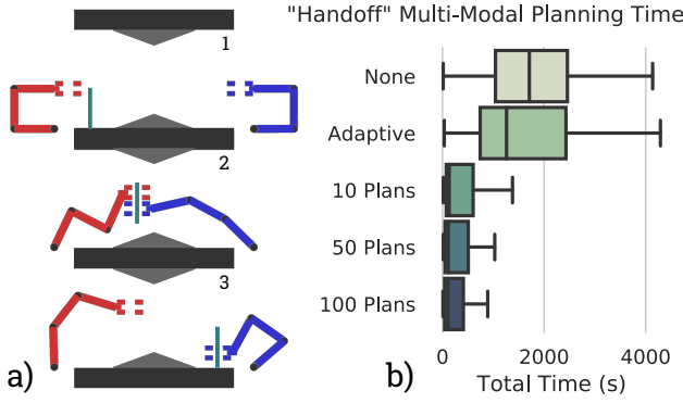
Fig. 10. a) Three stills from a multi-modal plan in the “handoff” environment. The thin object must be handed off to the far robot to reach the other side of the environment. Many motion plans are attempted in this environment, as the choice of parameterization determines if a handoff is possible. b) Total multi-modal planning time for 100 trials for each method, including training time for ALEF. Obstacles vary in position and rotation between each query. ALEF shows significant improvement over the baseline method.
