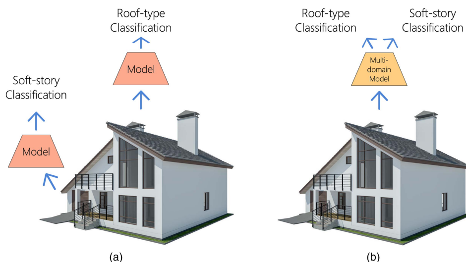
Fig. 1. Different approaches for information extraction from building images: (a) the baseline approach needs to train separate models for extracting different information from the building, which incurs large costs for training and storing the models; and (b) our proposed approach trains a single multidomain model for all the tasks with comparable accuracy to the baseline approach.
