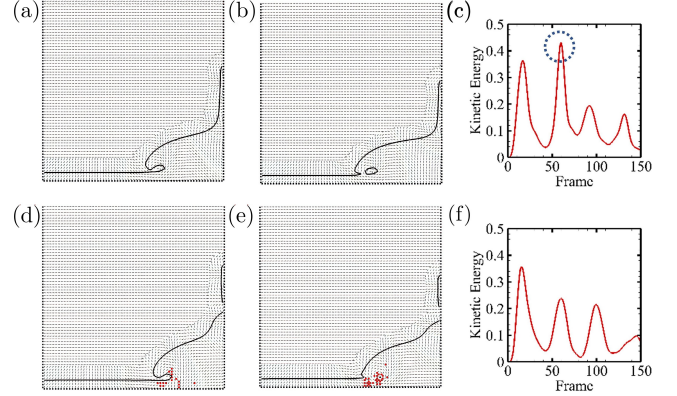
Fig. 12. Comparison of the wave-function distribution of a two-dimensional dam breaking (a), (b) without, and (d), (e) with wave-function correction. (a), (d) and (b), (e) are the two adjacent frames before and after the interface merge, respectively. (see the supplemented video for more details). We convert the first component of the two-component wave function to a vector in two-dimensional Euclidean space and plot it as an arrow line. Red points in (d) and (e) highlight the grid cells involved in the correction algorithm. (c) and (f) are the evolution of kinetic energy with and without wave-function correction, respectively. The dotted circle in (c) denotes a non-physical increment of kinetic energy without the correction step.
