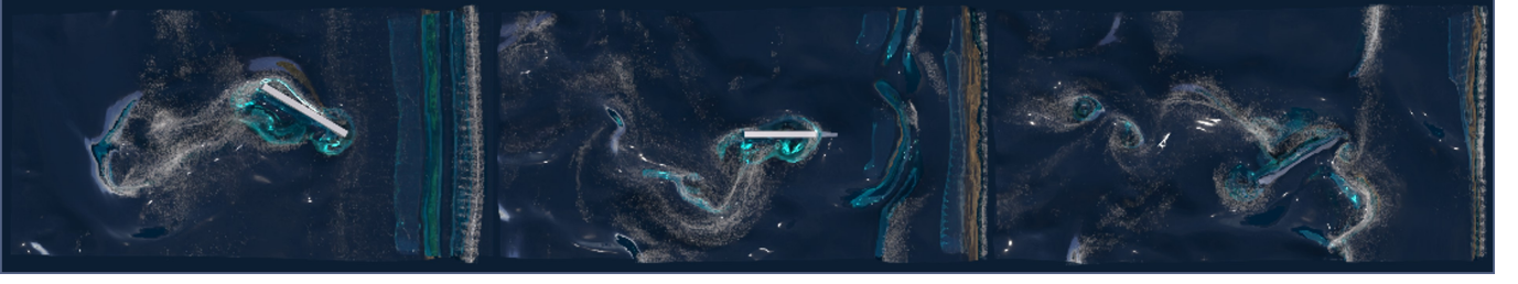
Fig. 10. A wiggling fishtail simulated on a sparse grid. The figures from left to right are frames 200, 550 and 900, respectively.
