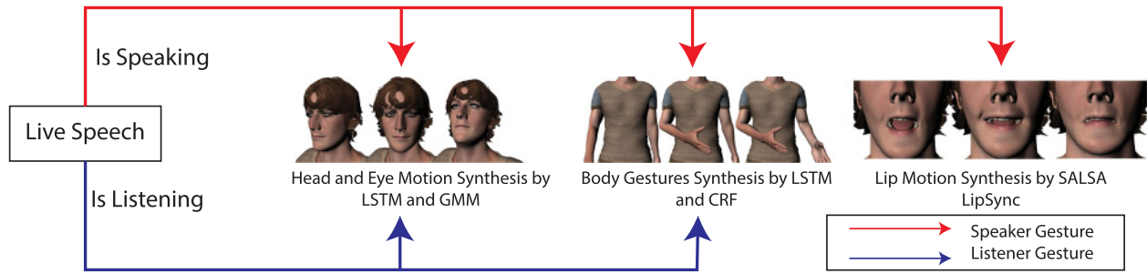
Figure 3. The pipeline of the motion synthesis components at each user's side in our system. We use a predefined intensity threshold to determine a user is speaking or listening at any moment and then call the corresponding motion synthesis modules. Here GMM stands for Gaussian Mixture Models.
