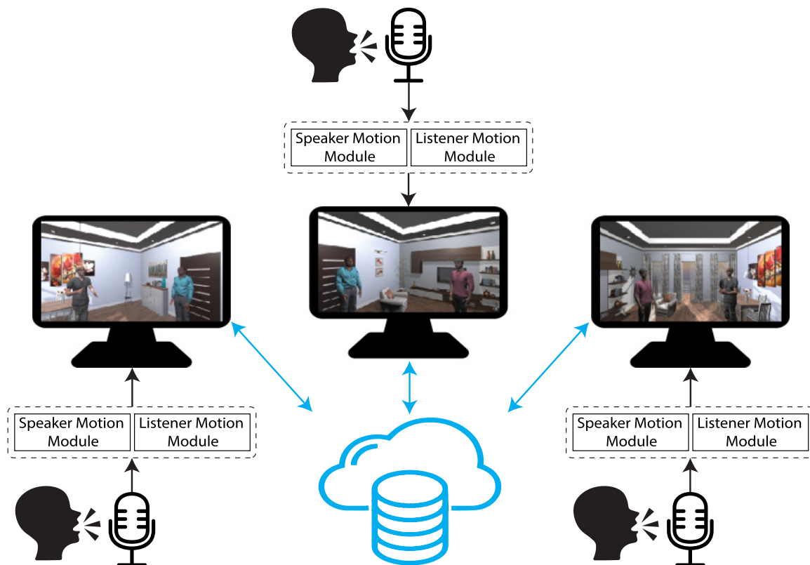
Figure 2. The architecture illustration of our system.
