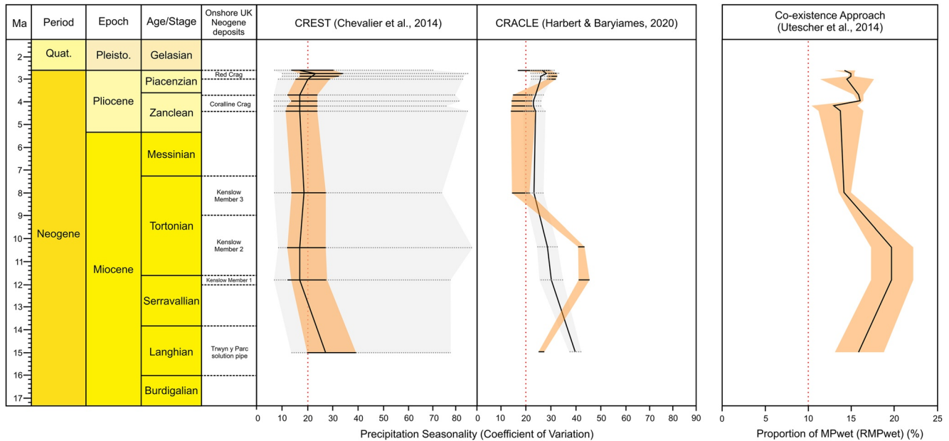
Figure 6. Precipitation Seasonality ( \text{CoV} \times 100 ) reconstructed by CREST, CRACLE compared to RMPwet (%) by the Co-existence Approach. CREST: 0.5 uncertainties in orange, 0.95 ( 2\sigma ) uncertainties in grey, optima represented by a solid black line. CRACLE: N-CRACLE 0.95 ( 2\sigma ) uncertainties in orange, P-CRACLE 0.95 ( 2\sigma ) uncertainties in grey, mean represented by a solid black line. Modern precipitation seasonality as a dotted red line (20). Co-existence Approach: proportion of MPwet (RMPwet) (%), mean represented by a solid black line. Modern RMPwet (10%) as a red dotted line.
