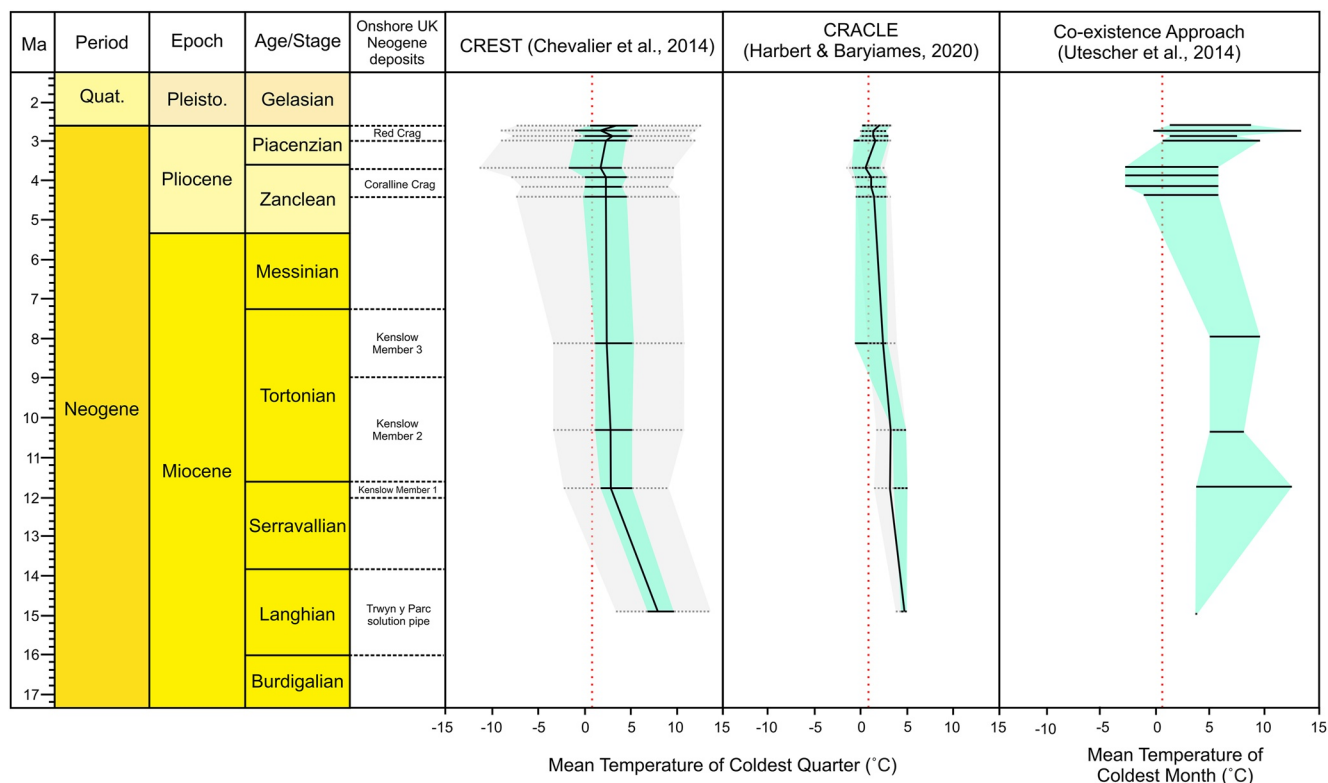
Figure 4. Mean Temperature of Coldest Quarter (MTCQ) reconstruction using CREST, CRACLE compared to Mean Temperature of the Coldest Month (MTCM) by the Co-existence Approach. CREST: 0.5 uncertainties in aqua, 0.95 ( 2\sigma ) uncertainties in grey, optima represented by a solid black line. CRACLE: N-CRACLE 0.95 ( 2\sigma ) uncertainties interval in aqua, P-CRACLE 0.95 ( 2\sigma ) uncertainties in grey, mean represented by a solid black line. Co-existence Approach: equal likelihood range in dark blue. Modern mean temperature of coldest month ( 1.4^{\circ}\text{C} ) as a dotted red line.
