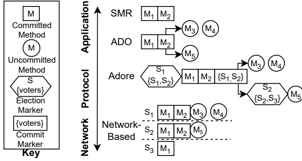
Figure 1. The spectrum of distributed system models. Each shows a snapshot of the same distributed state at a different level of abstraction. Network-based represents each node ( S_1, S_2, S_3 ) as a separate object. SMR and ADO treat the committed methods as a single, atomic object, but ADO also exposes uncommitted methods. ADORE is like ADO, but with additional evidence of the system’s safety in the form of election and commit markers that record the servers that approved each operation.
