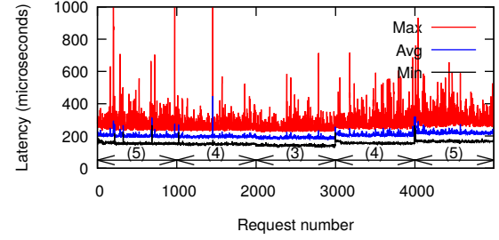
Figure 16. OCaml Raft performance under reconfiguration. ( n ) indicates a configuration under n nodes.
