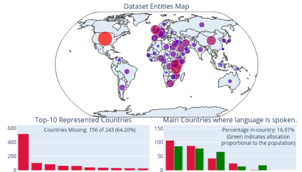
Swahili NER-Relaxed
