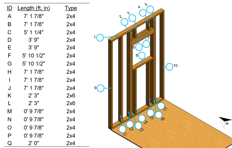
Figure 3. The worksheet where students assigned items on a list of pre-cut wood studs (left) to the numbered spaces on an isometric view of the completed wall (right).
