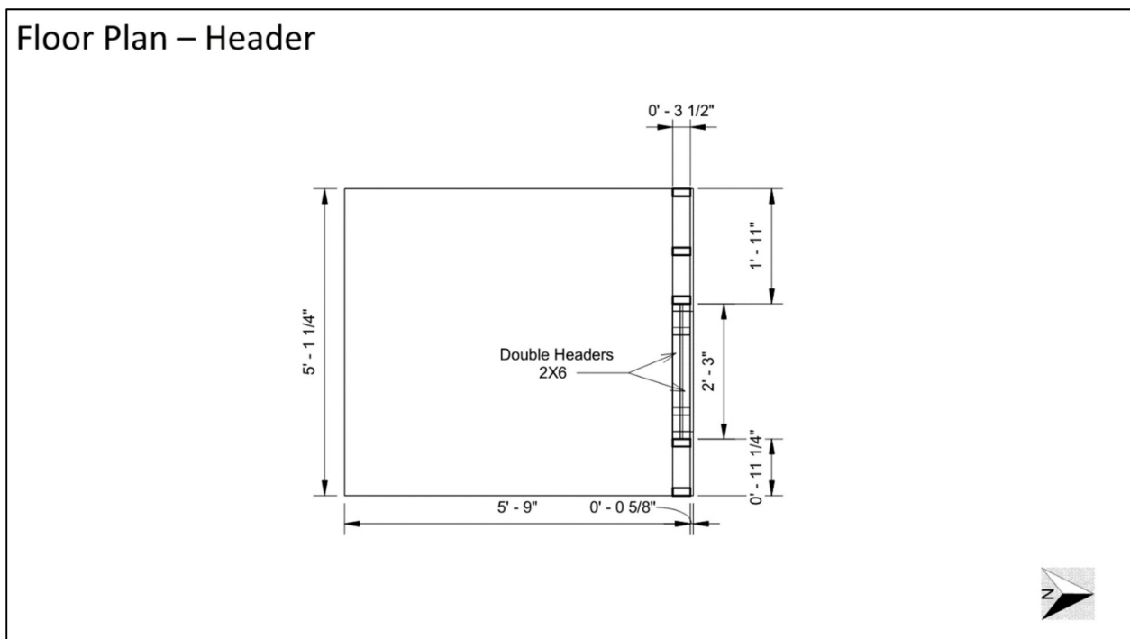
Figure A3. Header floor plan.
