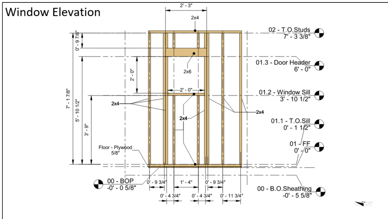
Figure A1. Window elevation.
