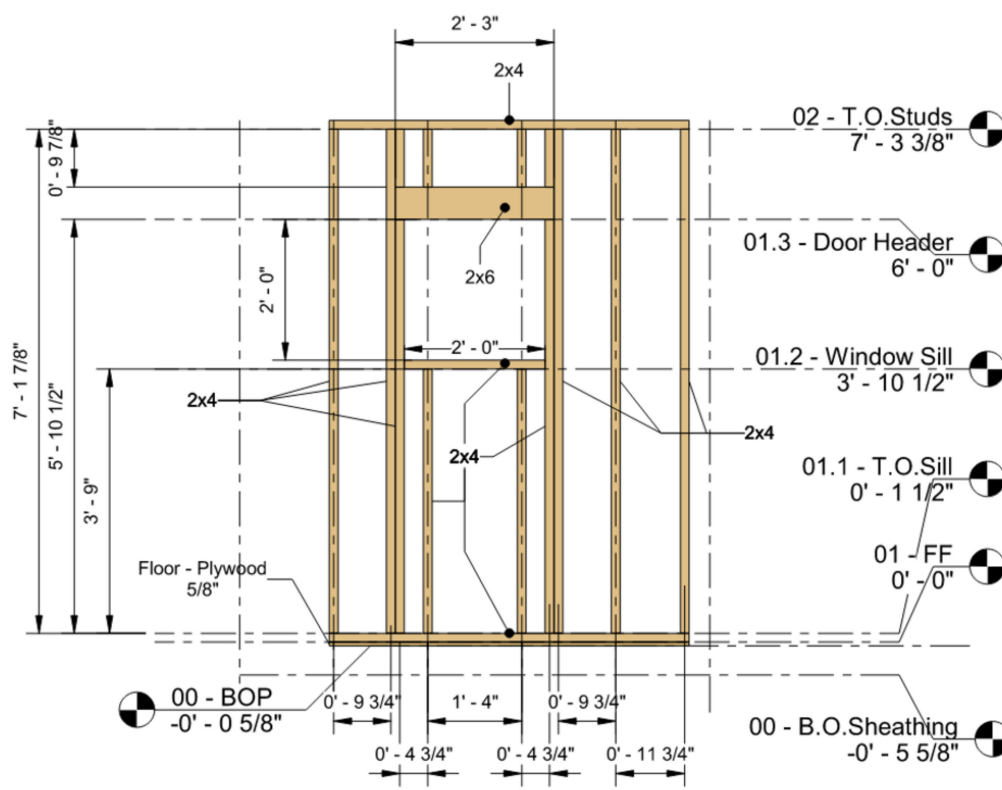
Figure 1. Example of one of the drawing sheets provided to students: a window elevation view of the framed wall. See the Appendix A for the full set of drawings.
