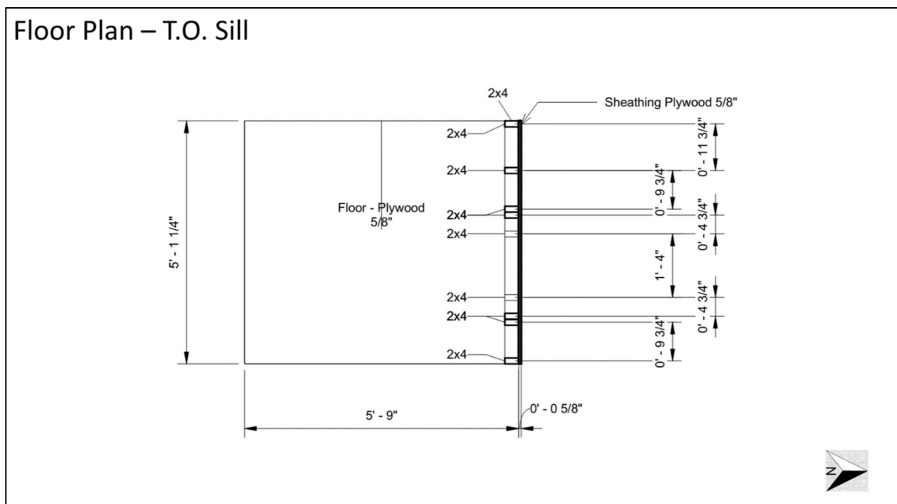
Figure A2. Top-of-sill floor plan.
