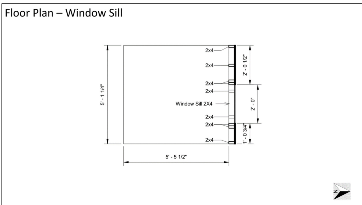
Figure A4. Windowsill floor plan.
