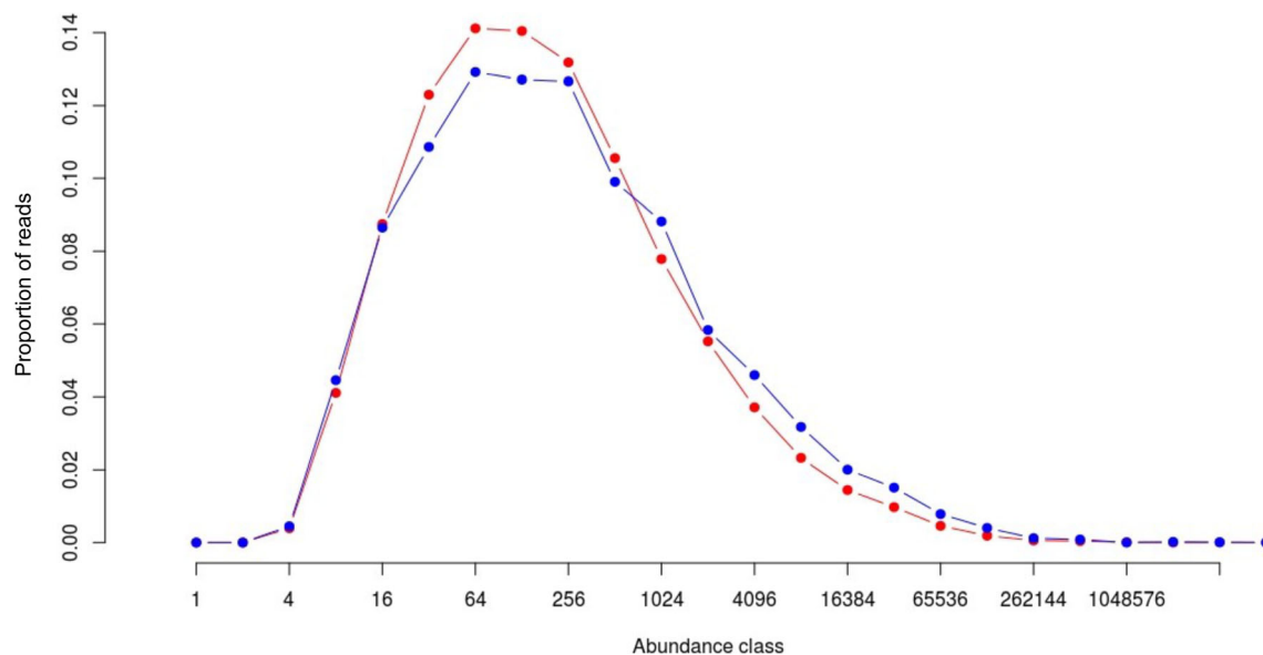
Fig. 4 Octave plot. Cluster abundance distributions for OTUs (in blue) and ASVs (in red). Cluster abundances are binned by octave or log base 2 increments meaning each octave contains OTUs or ASVs with double the abundance, measured by the number of reads, of the previous octave
