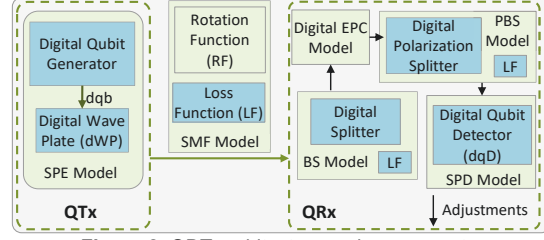
Figure 2. QDT architecture and components.
