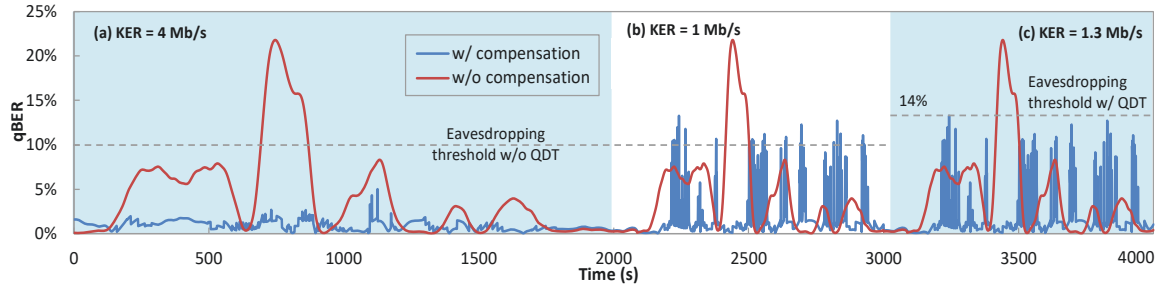
Figure 5. Improvement of the QKD using QDT.
