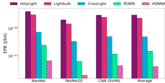
Figure 3: EPB for CNN models, across photonic accelerators.
