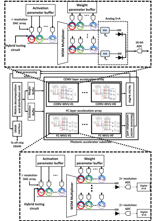
Figure 2: Architectural overview of HQNN with the internal architecture of CONV-MVU and FC-MVU highlighted.
