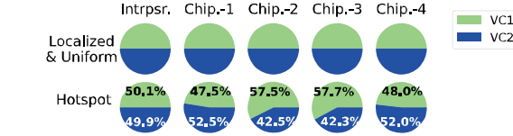
Figure 5. VC utilization in DeFT under synthetic traffic.
