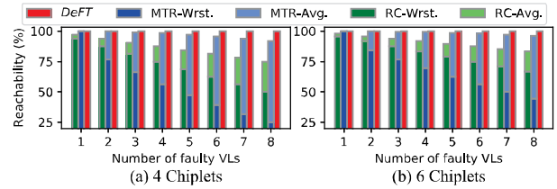
Figure 7. Reachability in the presence of VL faults in a system with (a) 4 chiplets (total VLs=32), and (b) 6 chiplets (total VLs=48). Note that DeFT -Wrst. and DeFT -Avg. are the same (both shown by DeFT ).
