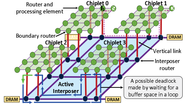
Figure 1. An abstract overview of the baseline 2.5D network with four chiplets on an active interposer.
