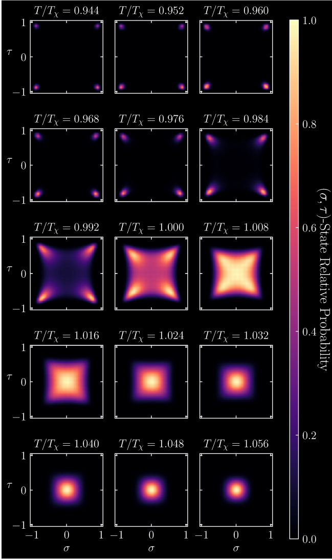
Figure 9. Relative thermodynamic probabilities of (\sigma, \tau) -states for the clean case with K = 0.5J . The central temperature corresponds to the peak \chi_{\sigma, \tau} position, T_\chi = 3.031J . The highest temperature is T = 3.2J .
