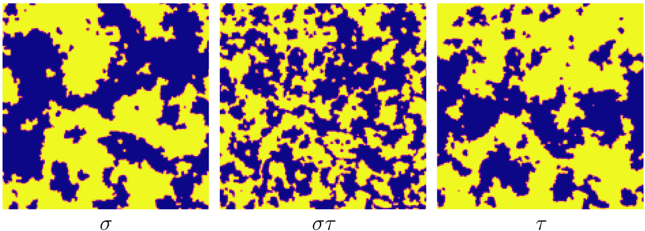
Figure 4. Snapshots of the low-temperature domain structure generated by a simulated annealing run of Eq. (8) for a single disorder configuration with K = 0 , \varepsilon = J , and L = 400 . The Baxter domains in the \sigma\tau panel are seen to be typically smaller than the magnetic domains in the \sigma and \tau panels. The yellow (light) regions are those for which the field values are +1 , whereas the blue (dark) regions correspond to -1 . The red lines highlight the domain walls.
