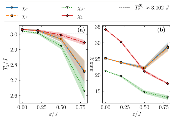
Figure 8. (a) Peak susceptibility temperature, T_\chi , and (b) peak susceptibility, \max \chi , as a function of disorder strength \varepsilon for K = 0.5 J and L = 40 . The shaded regions represent T_\chi and \max \chi within a single error bar. The lines are guides to the eye.
