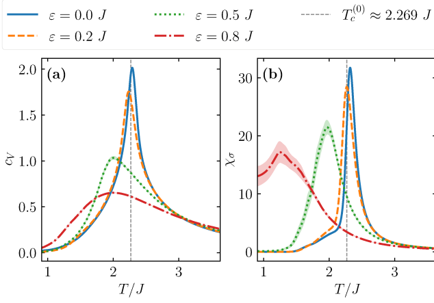
Figure 15. Disorder-averaged thermodynamic quantities of the RFIM with linear size L = 40 , measured as functions of temperature T , for various random field strengths \varepsilon . (a) The specific heat c_V . (b) The magnetic susceptibility \chi_\sigma .
