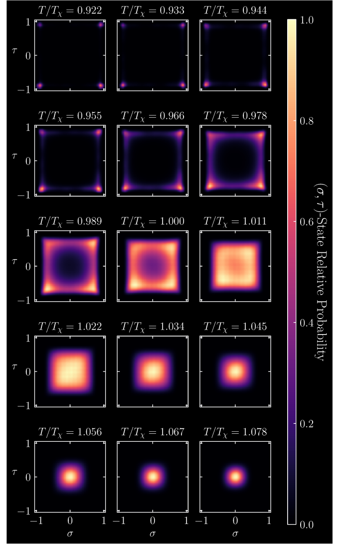
Figure 10. Relative thermodynamic probabilities of (\sigma, \tau) -states with K = 0.5J and a random Baxter field strength of \varepsilon = 0.5J . The central temperature corresponds to the peak \chi_{\sigma, \tau} position, T_\chi = 2.968J . The highest temperature is T = 3.2J , which is the same as Fig. 9.
