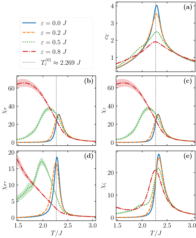
Figure 11. Temperature-dependence of (a) the specific heat c_V and (b-e) the uniform susceptibilities ( \chi ) of the RBFM for K = 0 and linear size L = 40 at different disorder strengths \varepsilon . The susceptibilities are labeled as follows: (b) \sigma susceptibility \chi_\sigma , (c) \tau susceptibility \chi_\tau , (d) the Baxter susceptibility \chi_{\sigma\tau} , and (e) the quadrature susceptibility \chi_\zeta .
