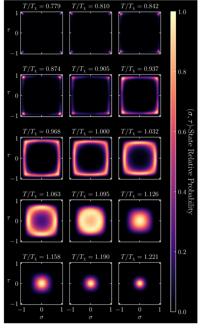
Figure 14. Relative thermodynamic probabilities of (\sigma, \tau) -states for K = 0 with \varepsilon = 0.5 J . The central temperature corresponds to the peak \chi_{\sigma, \tau} position, T_\chi = 2.129 J . The highest temperature is T = 2.6 J as it is in Fig. 13.
