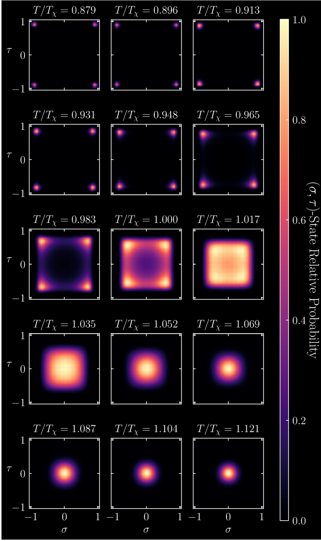
Figure 13. Relative thermodynamic probabilities of (\sigma, \tau) -states for the clean case for K = 0 . The central temperature corresponds to the peak \chi_{\sigma, \tau} position, T_\chi = 2.319 J . The highest temperature is T = 2.6 J .
