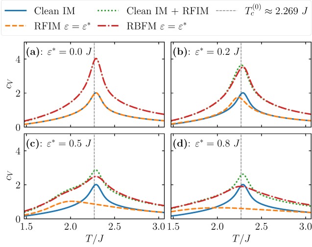
Figure 16. Comparison of the RFIM and the RBFM with L = 40 and K = 0 over various disorder strengths. These plots show the specific heat c_V as a function of temperature T for the clean Ising model (Clean IM); the RFIM at \varepsilon = \varepsilon^* , where \varepsilon^* is a numerical value defined in each figure; the sum of the specific heats of the Clean IM and the RFIM (Clean IM + RFIM); and the RBFM at zero Baxter coupling. (a) \varepsilon^* = 0.0 J , (b) \varepsilon^* = 0.2 J , (c) \varepsilon^* = 0.5 J , and (d) \varepsilon^* = 0.8 J . In the clean case (a), the Ashkin-Teller model is equivalent to two clean Ising models, as shown by the complete agreement between the green dotted curve and the red dash-dotted curve.
