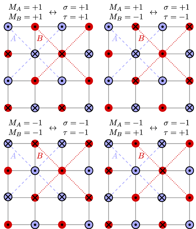
Figure 1. The fourfold degenerate stripe-magnetic ground state of the Ising J_1 - J_2 model on a square lattice. Blue and red sites denote the A and B sublattices. The magnetic moments point out of the plane. The horizontal (vertical) stripe configuration, corresponding to the ordering vector \mathbf{Q}_H = (0, \pi) ( \mathbf{Q}_V = (\pi, 0) ), corresponds to parallel (antiparallel) staggered sublattice magnetizations M_A and M_B . These states exhibit either a positive or negative nematic order parameter, defined as the product \phi \propto M_A M_B . The staggered magnetizations on the A and B sublattices of the Ising J_1 - J_2 model are in one-to-one correspondence with the \sigma and \tau Ising variables of the Ashkin-Teller model. Similarly, the nematic order parameter in the former maps onto the Baxter variable \sigma\tau of the latter.
