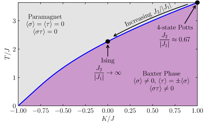
Figure 2. Two-dimensional phase diagram of the Ashkin-Teller model along the temperature T and Baxter coupling K axes, according to Ref. [56]. A critical line separates the paramagnetic phase from the Baxter phase, along which only one critical exponent is universal. The points displaying Ising ( K = 0 ) and 4-state Potts ( K = J ) universality are indicated, as is the mapping of the Ising J_1 - J_2 model with J_2/|J_1| \gtrsim 0.67 onto the 0 \leq K/J \leq 1 region of the phase diagram established in Refs. [47, 48].
