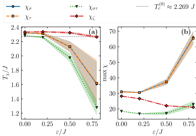
Figure 12. (a) Peak susceptibility temperature, T_\chi , and (b) peak susceptibility, \max \chi , as a function of disorder strength \varepsilon for K = 0 and L = 40 . The shaded regions represent T_\chi and \max \chi to within a single error bar. The lines are guides to the eye.
