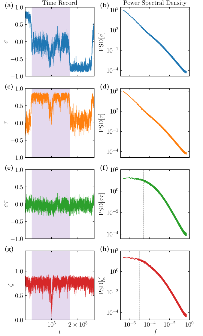
Figure 18. Metropolis evolution of the RBFM for a system size L = 80 , K = 0 , and \varepsilon = 0.5 J at the peak temperature from Fig. 12 ( T_\chi = 2.129 J ). We show a typical time record as a function of Monte Carlo sweeps t and the disorder-averaged power spectral density (PSD) as a function of frequency f for the (a, b) \sigma , (c, d) \tau , (e, f) Baxter \sigma\tau , and (g, h) quadrature \zeta variables. The vertical lines correspond approximately to the frequencies at which the PSDs crossover from a plateau to a power-law behavior, if plateaus are present. The highlighted region of the time records is discussed in the main text.
