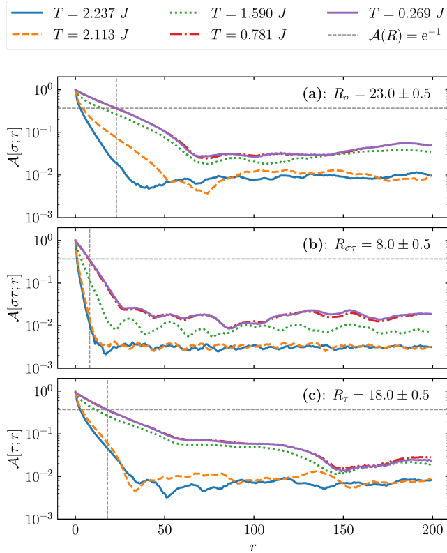
Figure 5. Isotropic spin autocorrelation functions \mathcal{A}(r) of snapshots of the spin configurations taken after equilibration at various temperatures during simulated annealing. These autocorrelations are of the (a) \sigma , (b) Baxter \sigma\tau , and (c) \tau degrees of freedom and are measured with respect to the radial coordinate r = \sqrt{x^2 + y^2} . The vertical lines are positioned at the radius R where \mathcal{A}(R) = e^{-1} at the lowest temperature probed.
