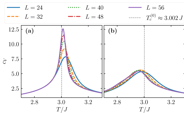
Figure 7. Comparison of the specific heat c_V of (a) the clean system ( \varepsilon = 0 ) and (b) the disordered system ( \varepsilon = 0.5 J ) with increasing system size L . The Baxter coupling for both cases was set to K = 0.5 J .
