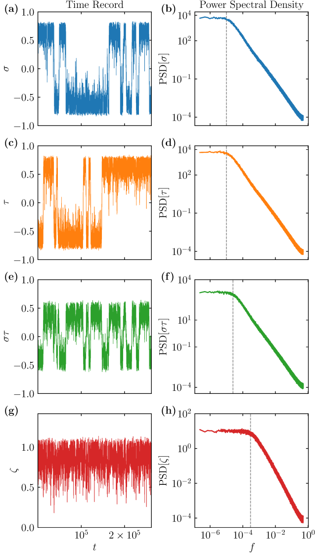
Figure 17. Metropolis evolution of the RBFM for a system size L = 80 and K = 0 for the clean case ( \varepsilon = 0 ) at the transition temperature T_c^{(0)} \approx 2.269 J . We show a typical time record as a function of Monte Carlo sweeps t and the average power spectral density (PSD) as a function of frequency f for the (a, b) \sigma , (c, d) \tau , (e, f) Baxter \sigma\tau , and (g, h) quadrature \zeta variables. The vertical lines correspond approximately to the frequencies at which the PSDs crossover from a plateau to a power-law behavior.
