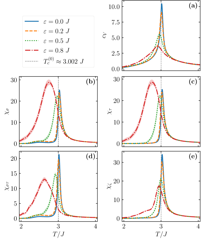
Figure 6. Temperature dependence of (a) the specific heat c_V and (b-e) the uniform susceptibilities of the RBFM for K = 0.5 J and linear size L = 40 at different disorder strengths \varepsilon . The susceptibilities are labeled as follows: (b) \sigma susceptibility \chi_\sigma , (c) \tau susceptibility \chi_\tau , (d) the Baxter susceptibility \chi_{\sigma\tau} , and (e) the quadrature susceptibility \chi_\zeta .
