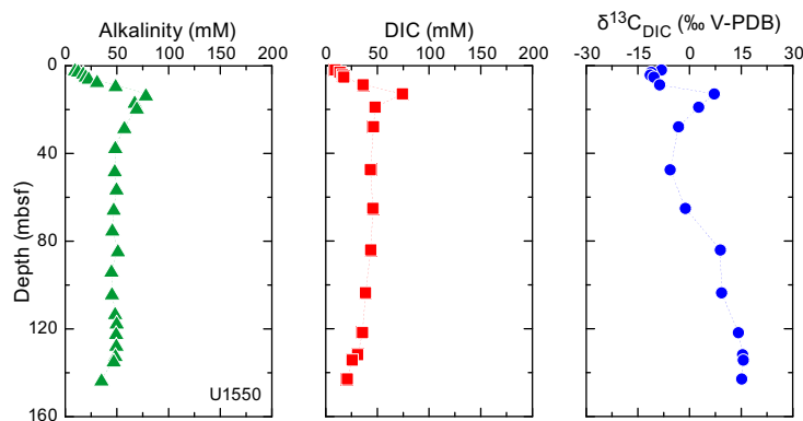
Figure F5. Downcore profiles of alkalinity, DIC, and \delta^{13}\text{C}_{\text{DIC}} Site U1550. Alkalinity data from Teske et al. (2021g). V-PDB = Vienna Pee Dee belemnite.
