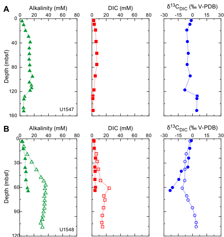
Figure F3. Downcore profiles of alkalinity, DIC, and \delta^{13}\text{C}_{\text{DIC}} . Sites (A) U1547 and (B) U1548. Solid symbols = Hole U1548C, open symbols = Hole U1548D. Alkalinity data from Teske et al. (2021e). V-PDB = Vienna Pee Dee belemnite.
