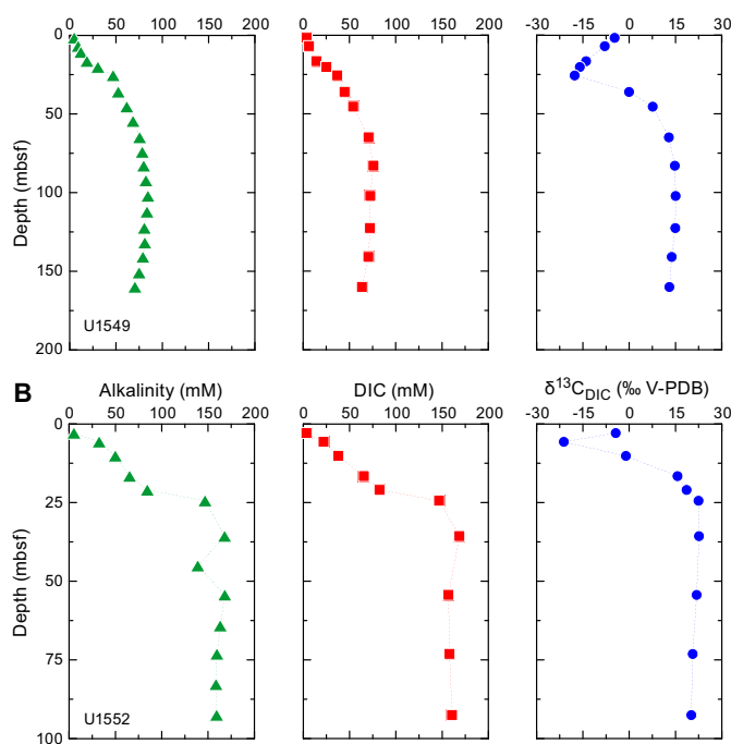
Figure F4. Downcore profiles of alkalinity, DIC, and \delta^{13}\text{C}_{\text{DIC}} Sites (A) U1549 and (B) U1552. Alkalinity data from Teske et al. (2021f, 2021h). V-PDB = Vienna Pee Dee belemnite.
