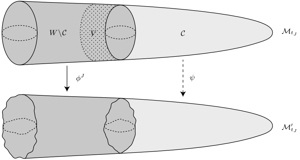
Figure 7. Extending the map \phi^J_{W \setminus C} over the extension cap C to an almost isometry \psi: W \rightarrow W' .
