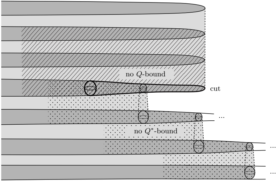
Figure 9. The bound Q \leq \bar{Q} in (APA7) holds on all of \mathcal{N} except for the hatched region. The bound Q^* \leq \bar{Q}^* in (APA9) holds on all of \mathcal{N} except for the dotted region.
