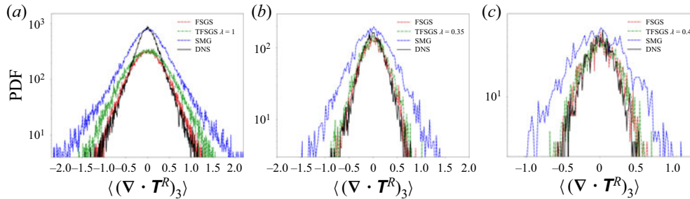
Figure 7. Probability density function of the ensemble-averaged \langle \nabla \cdot \mathbf{T} \rangle_{i=3} for the optimized (tempered) fractional and the SMG models at (a) \mathcal{L}_\delta = 4 , (b) \mathcal{L}_\delta = 8 and (c) \mathcal{L}_\delta = 12 .
