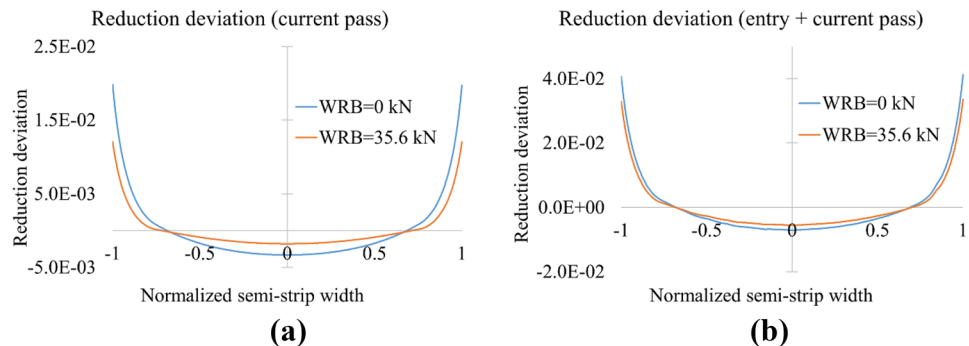
Fig. 18 a Reduction deviation induced in the current pass and b total reduction deviation of SS 301 thin gauge (0.236 mm)
