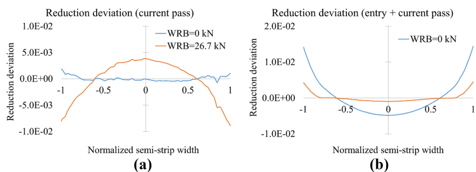
Fig. 16 a Reduction deviation induced in the current pass and b total reduction deviation of Al 6061-O thick gauge (2.576 mm)
