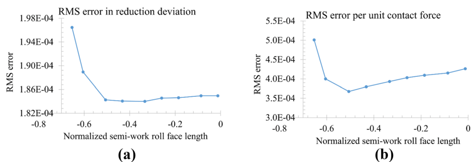
Fig. 14 a RMS error in reduction deviation for a single deviation at different locations; b corresponding RMS value per unit normalized rolling force
