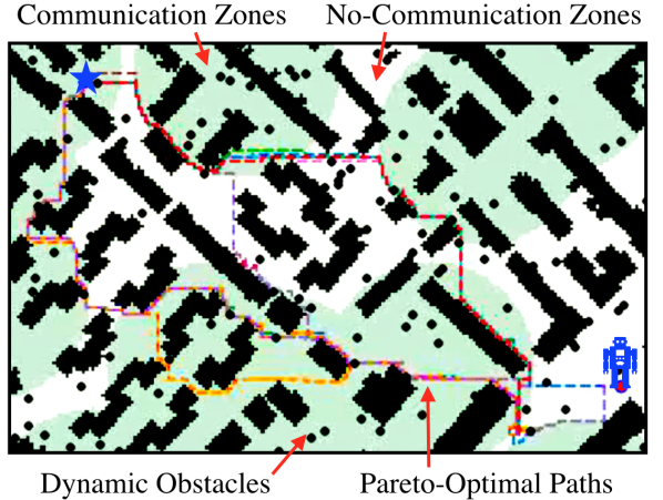
Fig. 1: A motivating example of MOPPwDO in the context of urban search and rescue. A robot needs to plan collision-free paths among dynamic obstacles in a city-like map while optimizing the arrival time and communication robustness along the path. For paths with smaller arrival times, the robot may have to traverse regions with no communication (the white area). Computing a Pareto-optimal set of solutions can reveal the underlying trade-off between different objectives and can potentially help decision makers to better understand the mission and make informed decisions.
