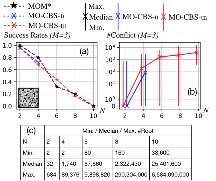
Fig. 5: Comparison among MO-CBS-n, MO-CBS-tn, MOM* with M = 3 (fixed) and varying N in the random 32x32 map. When M increases from 2 to 3, the problem instances become more challenging and the success rates decrease for all three planners.
