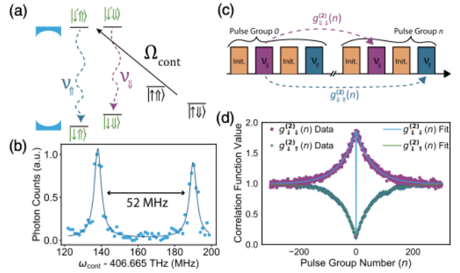
FIG. 5. (a) Hyperfine splitting due to the ^{29}\text{Si} nuclear spin gives rise to a four-level ground-state manifold. Pumping on the electron-spin-flipping transition with \Omega_{\text{cont}} results in the generation of photons with two nuclear-state-dependent frequencies \nu_{\uparrow\uparrow} and \nu_{\downarrow\downarrow} . (b) Sweeping the control pulse frequency selectively tunes \nu_{\uparrow\uparrow} and \nu_{\downarrow\downarrow} into resonance with the filter cavity, which enables the measurement of the spectrum of the emitted photons. (c) Pulse sequence for attempting to measure two consecutive photons either at nuclear-state dependent frequencies \nu_{\downarrow\downarrow} and \nu_{\downarrow\downarrow} , or at nuclear-state dependent frequencies \nu_{\downarrow\downarrow} and \nu_{\uparrow\uparrow} . (d) Purple: g_{\downarrow\downarrow}^{(2)}(\tau) autocorrelation measurements of the photons emitted at \nu_{\downarrow\downarrow} show antibunching at zero time delay, and bunching after the emission of 113.8 \pm 3.8 photons (1.48 ms timescale). Blue: g_{\downarrow\uparrow}^{(2)}(\tau) cross-correlation function for the two consecutively emitted photons at \nu_{\uparrow\uparrow} and \nu_{\downarrow\downarrow} shows antibunching after the emission of 110.6 \pm 2.4 photons, suggesting that the nuclear polarization is preserved for repeated generation of up to 110 photons.
