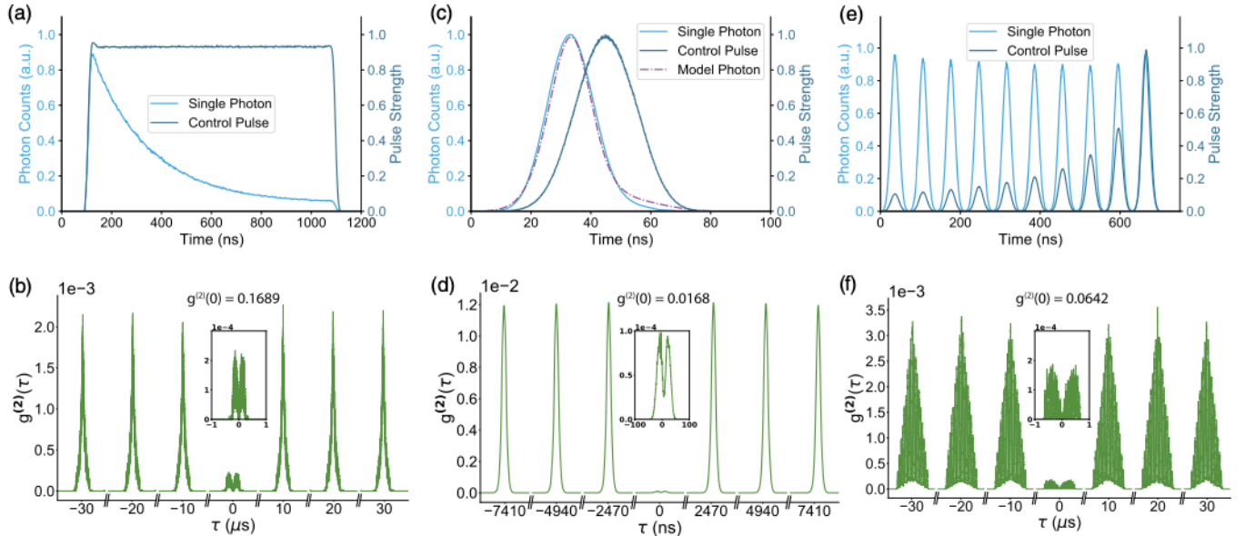
FIG. 3. Pulse-shaped single-photon generation. The upper panels (a), (c), (e) display the temporal profile of the coherent control pulse and detected single photon. (a) A square control pulse produces an exponentially decaying photon. (c) A Gaussian single photon. (e) A single photon distributed over ten time bins. The lower panels (b), (d), (f) display the normalized second-order correlation of photon arrivals for the exponential, Gaussian, and ten-peaked photons, respectively. The insets show a zoomed-in window around \tau = 0 , which is integrated to calculate g^{(2)}(0) .
