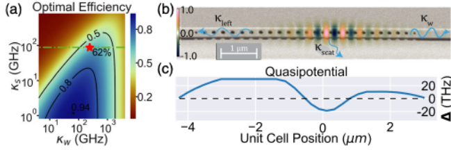
FIG. 2. (a) Photon extraction efficiency is shown in the color plot as a function of cavity-waveguide coupling \kappa_w and unwanted cavity loss rate \kappa_s . Contours aid readability of the color map. Optimal extraction efficiency is maximized by trading off atom-photon interaction probability, proportional to (\kappa_s + \kappa_w)^{-1} , for a higher cavity-waveguide coupling rate \kappa_w . The dash-dotted line cut corresponds to \kappa_s = 89 GHz, the unwanted loss rate of this device, which is determined by fabrication imperfections. The red star highlights this device with waveguide coupling rate \kappa_w = 240 GHz, which is nearly optimal for the given \kappa_s . (b) A scanning electron micrograph (SEM) of the nanophotonic cavity is overlaid with the simulated electric field, and loss rates are labeled, where \kappa_s = \kappa_{\text{scat}} + \kappa_{\text{left}} . (c) The simulated quasipotential shape of the cavity (see Sec. I.1 in the Supplemental Material [35]) shows that there is a lower and shorter potential barrier on the weak mirror side. This corresponds to the coupling to the right waveguide being the dominant loss rate ( \kappa_w \gg \kappa_s ).
