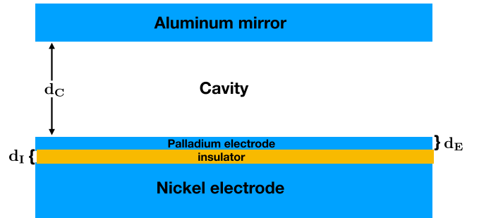
FIG. 1. An optical cavity of thickness d_C is bounded by an aluminum mirror and a M - I - M interface. The latter consists of a nickel electrode, a palladium electrode of thickness d_E , and a layer of insulator of thickness d_I .
