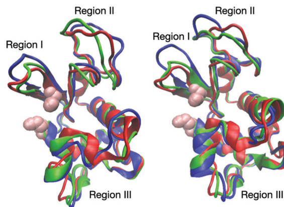
Fig. 3 The alignment of the average structures from water (red), 50 wt% ILs (blue) and rehydrated (green) systems in [EMIM][EtSO 4 ] (left) and [EMIM][Et 2 PO 4 ] (right). Pink vdW representations are the active site residues (residue 35 and 52). The high RMSF regions are also indicated.
