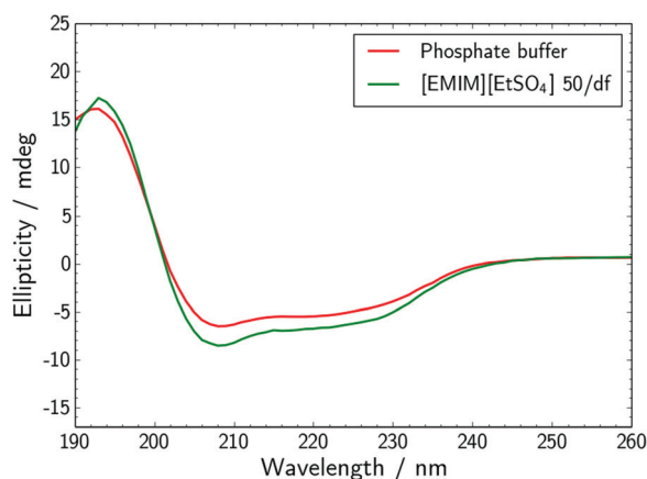
Fig. 1 Far-UV CD spectra of lysozyme. Freshly prepared sample in phosphate buffer (red), freshly prepared in 50 wt% [EMIM][EtSO 4 ] and rehydrated with water (green) and sample aged in 50 wt% [EMIM][EtSO 4 ] and rehydrated with water (green dashed). The dilution factor df = 1000 .
