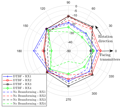
Fig. 4. Measured receive power at the four UAV-mounted receive antennas across all rotation angles and 0° induced phase offset. Solid lines indicate Rx power when DTBF and dashed lines indicate no beamforming.
