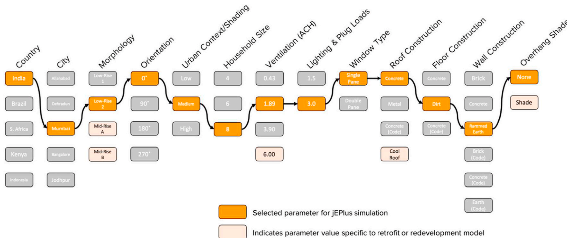
Fig. 3. Example of an energy modeling parameter tree representing simulation scenarios for informal settlements in India. For each energy simulation, the model takes a unique combination of each column of parameter values. Each country’s parameter tree may differ from one another based on its localized set of building materials.
