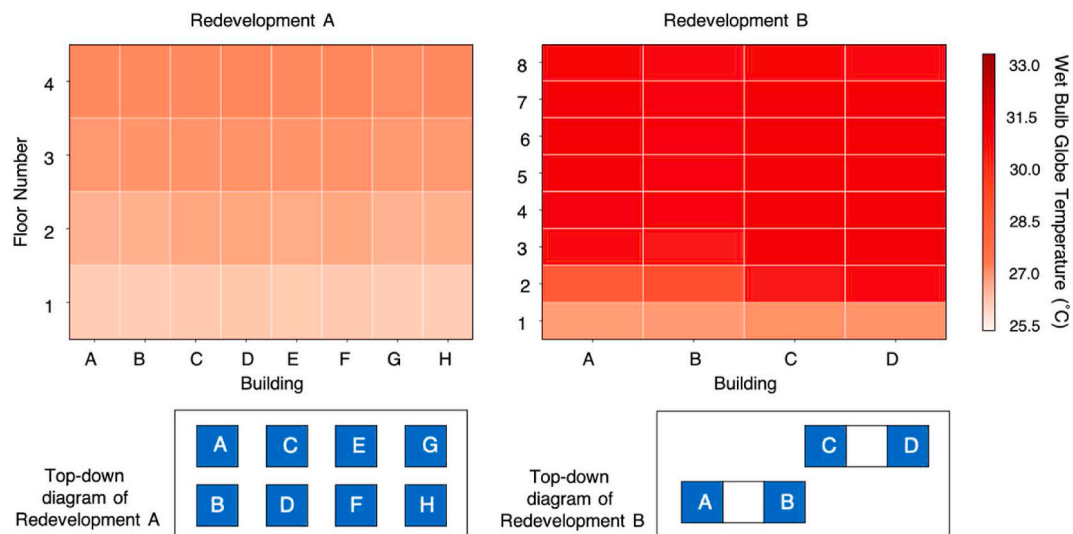
Fig. 10. Median WBGT by dwelling for Redevelopment Options A and B in Mumbai, India. The redevelopment options are based on designs proposed by Mumbai's Informal settlement Redevelopment Authority [97] that represent mid-rise morphologies constructed under building code-compliant construction materials.
