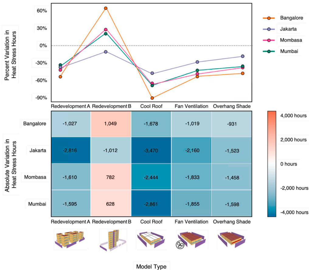
Fig. 8. Variation (percentage reduction, top; absolute reduction bottom) of annual heat stress incidents (hours during the year when wet bulb globe temperature (WBGT) is less than 35 °C for at least 4 hours) of each retrofit/redevelopment type when compared to Baseline model conditions.
