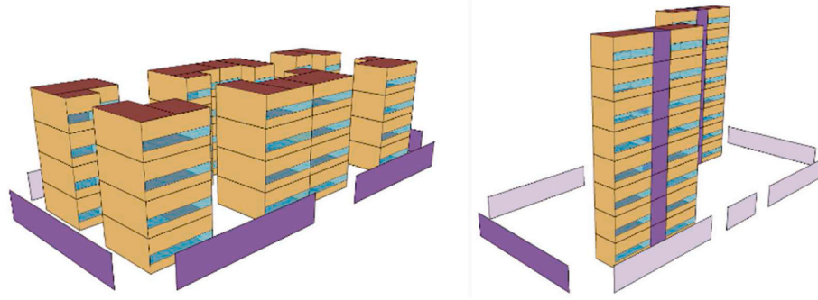
Fig. 4. Mid-rise redevelopment morphologies. These building geometries are modeled after designs from Ref. [12]. Like Fig. 2, the purple structures surrounding these models also represent urban shading that capture the impacts of how surrounding buildings may affect the informal settlements year-round.
