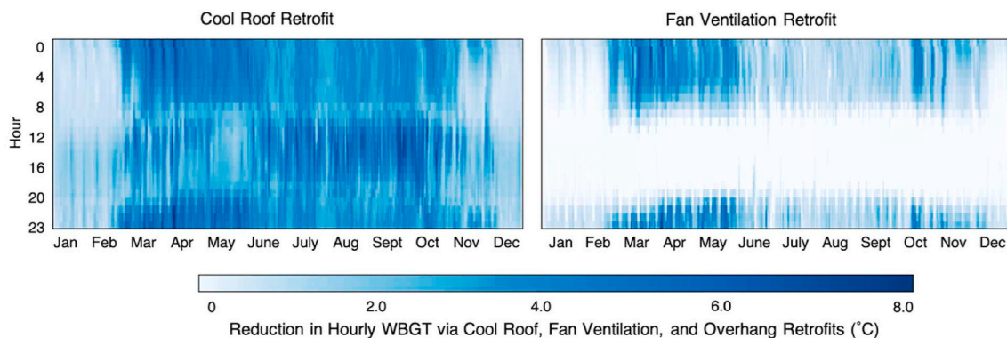
Fig. 9. Reduction in hourly wet bulb globe temperature (WBGT) in Mumbai, India when retrofitting Baseline models to cool roofs (left) and increased ventilation (right). Details on retrofit modeling assumptions are described in Section 3.5.
