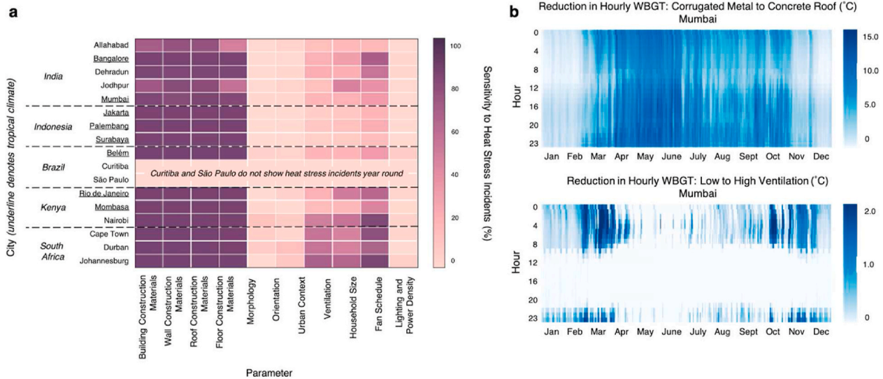
Fig. 7. (a) Sensitivity to annual changes in heat stress exposure by urban and building-level design parameters. (b) Reduction in hourly WBGT in Mumbai, India when modifying a single design parameter in the Baseline model: metal to concrete roof (top) and low to high ventilation levels (bottom).
