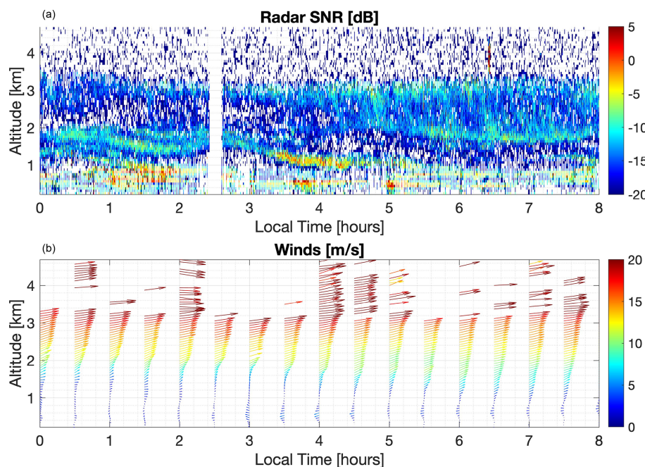
Figure 3. Example measurements by the LAP3000 915 MHz radar wind profiler showing SNR (a) and wind barbs (b) for 6 November from 00:00–08:00 LT. The radar is briefly turned off periodically for maintenance – seen as a pause between 02:00 and 03:00 LT.
