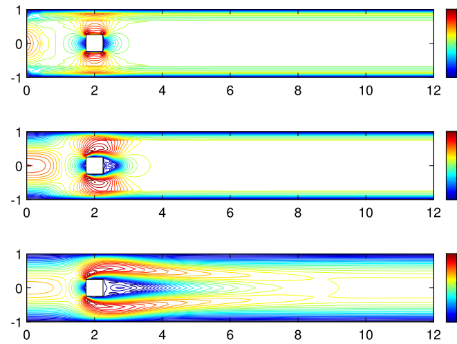
Fig. 4.9. Mean horizontal velocity at times 0.1 s (top), 1 s (center) and 10 s (bottom) for mean Reynolds number Re_1 = 300 and CoV = 1\% .
