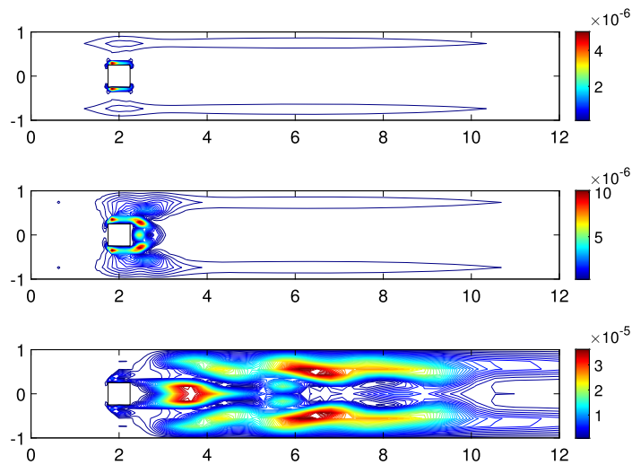
Fig. 4.10. Variance of the horizontal velocity at times 0.1 s (top), 1 s (center) and 10 s (bottom) for mean Reynolds number Re_1 = 300 and CoV = 1\% .
