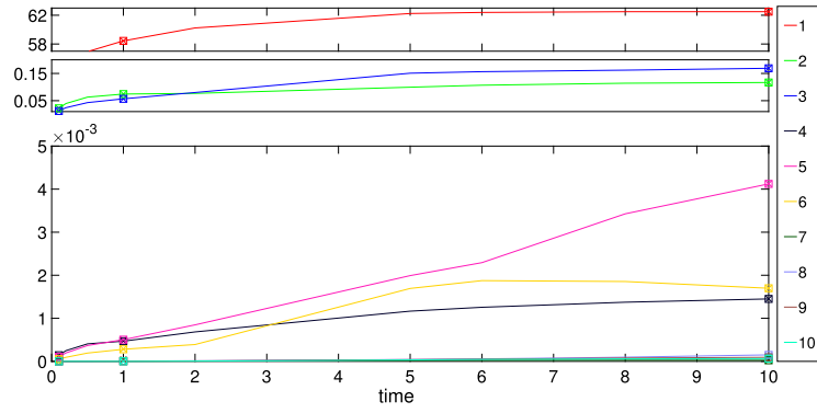
Fig. 4.8. Evolution of the gPC coefficients corresponding to the horizontal velocity in terms of \ell_2 -norm for mean Reynolds number Re_1 = 300 and CoV = 1\% . The symbols \square and \times represent the results of the Monte Carlo and stochastic collocation, respectively, at times 0.1 s, 1 s and 10 s.
