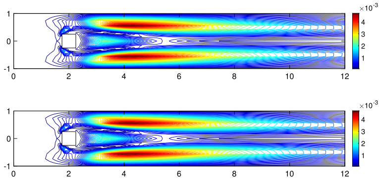
Fig. 4.14. Variance of the horizontal velocity obtained using the stochastic Galerkin methods for the steady-state problem (top), and at time 100 s (bottom) with mean Reynolds number Re_1 = 100 and CoV = 10\% .
