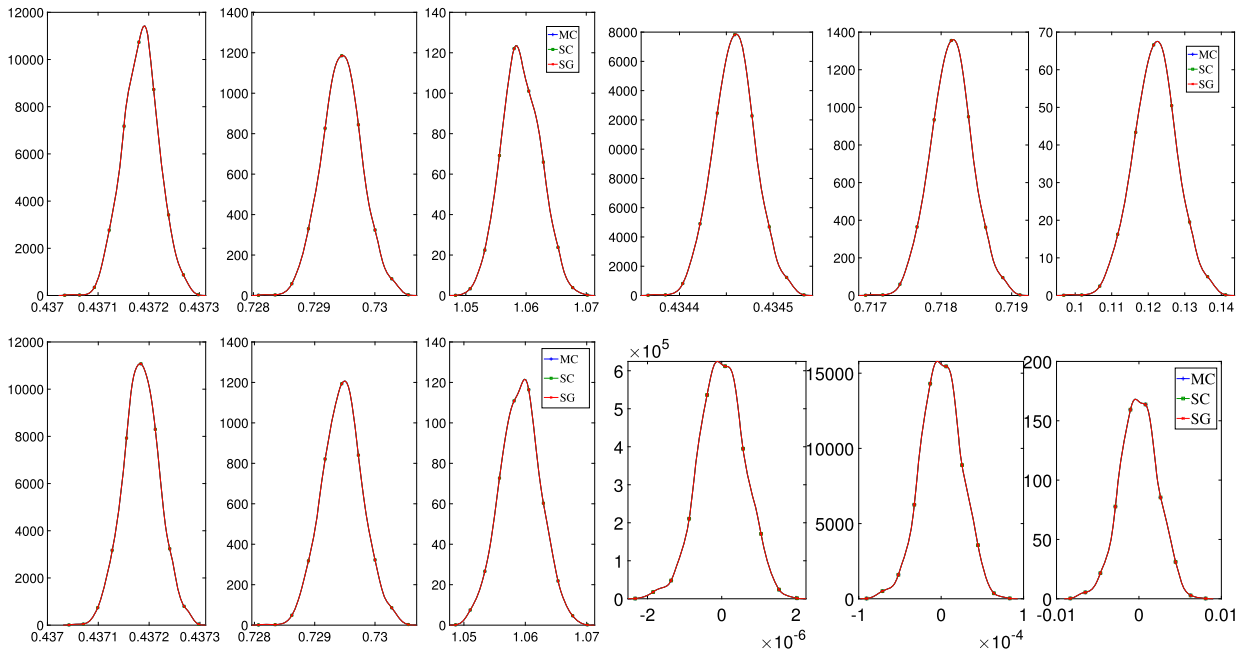
Fig. 4.12. Estimated probability density functions at times 0.1 s, 1 s and 10 s (left to right, all panels) of the horizontal velocity at points with coordinates (4.0100, -0.4339) (top left), (4.0100, 0.4339) (bottom left), and of the horizontal (top right) and vertical (bottom right) velocities at the point (3.6436, 0) for mean Reynolds number Re_1 = 300 and CoV = 1\% .
