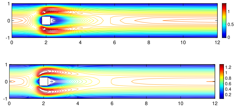
Fig. 4.13. Mean horizontal velocity obtained using the stochastic Galerkin methods for the steady-state problem (top), and at time 100 s (bottom) with mean Reynolds number Re_1 = 100 and CoV = 10\% .
