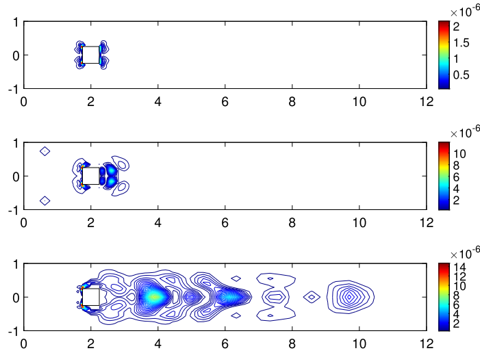
Fig. 4.11. Variance of the vertical velocity at times 0.1 s (top), 1 s (center) and 10 s (bottom) for mean Reynolds number Re_1 = 300 and CoV = 1\% .
