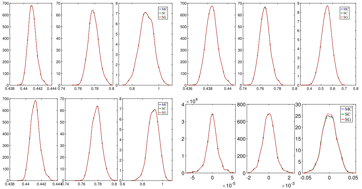
Fig. 4.7. Estimated probability density functions at times 0.1 s, 1 s and 10 s (left to right, all panels) of the horizontal velocity at points with coordinates (4.0100, -0.4339) (top left), (4.0100, 0.4339) (bottom left), and of the horizontal (top right) and vertical (bottom right) velocities at the point (3.6436, 0) for mean Reynolds number Re_1 = 100 and CoV = 10\% .
