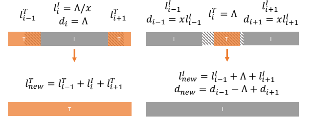
FIG. 3. RG rules. A pictorial representation of MHI RG rules. Each I-block is characterized by a deficit d_i (represented by the striped region) and a physical length l_i^I (striped plus gray region), while each T-block is characterized by a single physical length l_i^T (the orange region). On the LHS, the T-blocks are longer than the striped region and a TIT \rightarrow T follows. On the RHS, the T-block in the middle is shorter than the striped region and a ITI \rightarrow I ensues.
