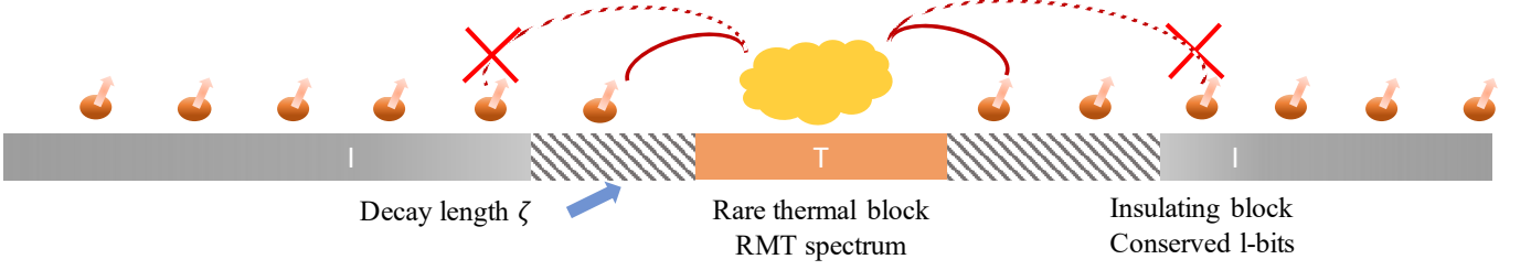
FIG. 2. Avalanche picture. The T-blocks are treated as thermal baths satisfying ETH (the yellow clouds represent a swarm of scrambled microscopic degrees of freedom). The I-blocks are a chain of exponentially localized I-bits. The red curves represent the exponentially decaying interactions (with decay length \zeta represented by the striped regions) between bath degrees of freedom and I-bits in I-blocks. When \zeta is too large, the bath degrees of freedom thermalize the I-bits closest to boundary, thus growing the T-block length until the entire I-block is absorbed. When \zeta is small, the T-block cannot reach far beyond the boundary and the surrounding I-blocks remains insulating. This is the basic physical picture for the quantum avalanche introduced in Ref. 43.
