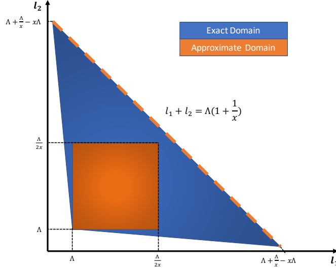
FIG. 6. In this plot we show the exact and approximate integration domains relevant for the production term. The opening angle of the isosceles triangle (exact domain) approaches \pi/2 as x \rightarrow 0 .
