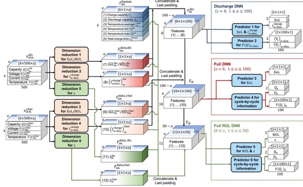
Fig. S 2: The workflow of the three DNNs in the current work. Where cubes represent data in tensor form and rounded rectangles represent neural networks.
