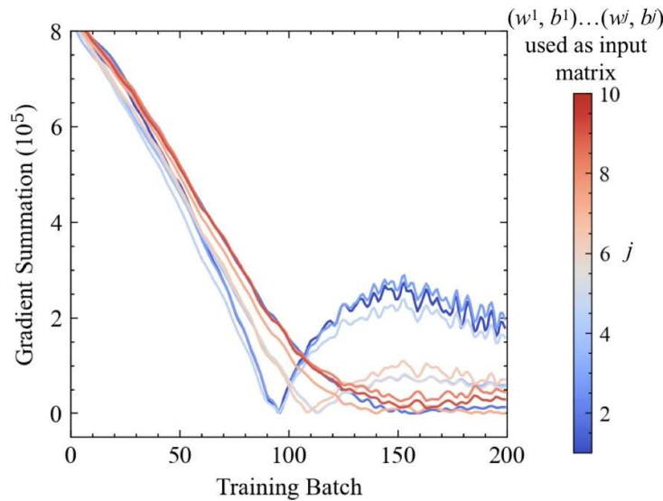
Fig. S 30: The gradient summation contributed by the j -th input matrix in each training batch.
