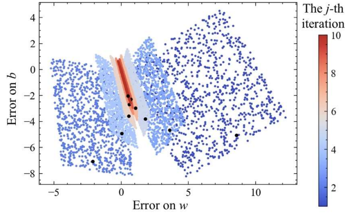
Fig. S 28: The error of w and b of 1000 lines in the j -th iteration. Where the black dots show the path of the convergence of one of the lines, showing the error dramatically altered between the iterations
